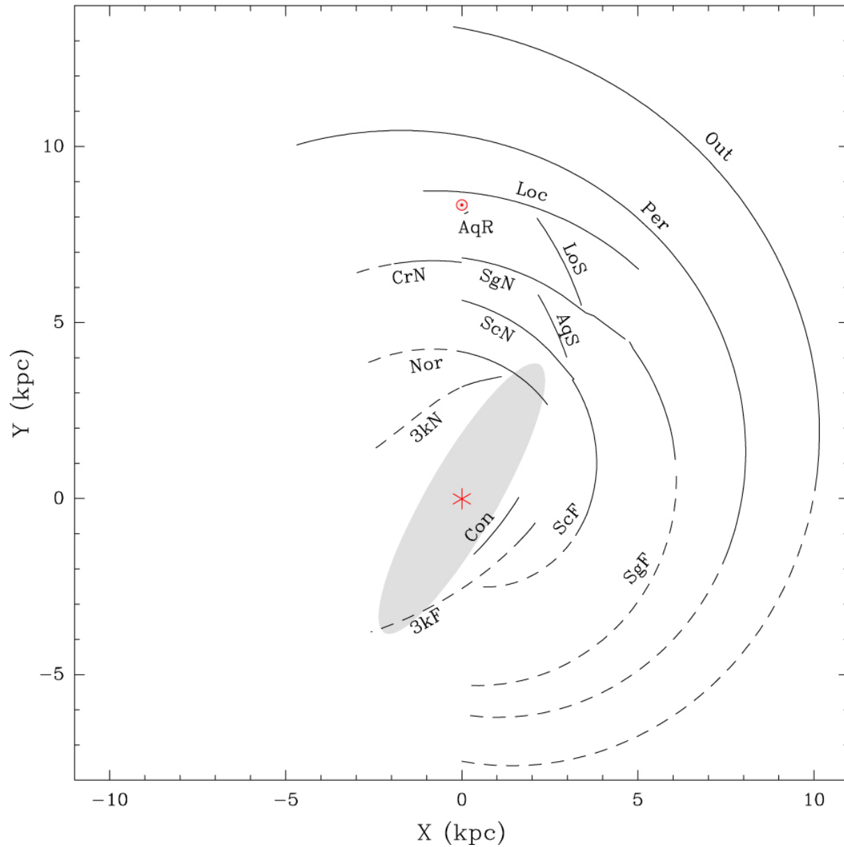
Figure 1. from A PARALLAX-BASED DISTANCE ESTIMATOR FOR SPIRAL ARM SOURCES null 2016 APJ 823 77 doi:10.3847/0004-637X/823/2/77 https://dx.doi.org/10.3847/0004-637X/823/2/77 © 2016. The American Astronomical Society. All rights reserved.
