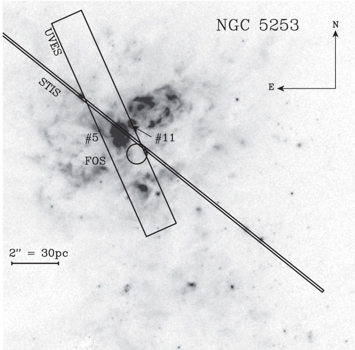
Figure 2. from THE VERY MASSIVE STAR CONTENT OF THE NUCLEAR STAR CLUSTERS IN NGC 5253 null 2016 APJ 823 38 doi:10.3847/0004-637X/823/1/38 https://dx.doi.org/10.3847/0004-637X/823/1/38 © 2016. The American Astronomical Society. All rights reserved.
