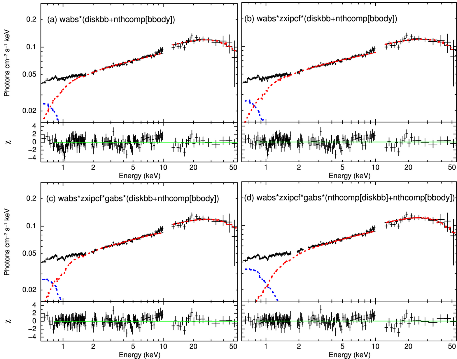
Figure 3. from SUZAKU OBSERVATION OF THE HIGH-INCLINATION BINARY EXO 0748–676 IN THE HARD STATE null 2016 APJ 823 131 doi:10.3847/0004-637X/823/2/131 https://dx.doi.org/10.3847/0004-637X/823/2/131 © 2016. The American Astronomical Society. All rights reserved.
