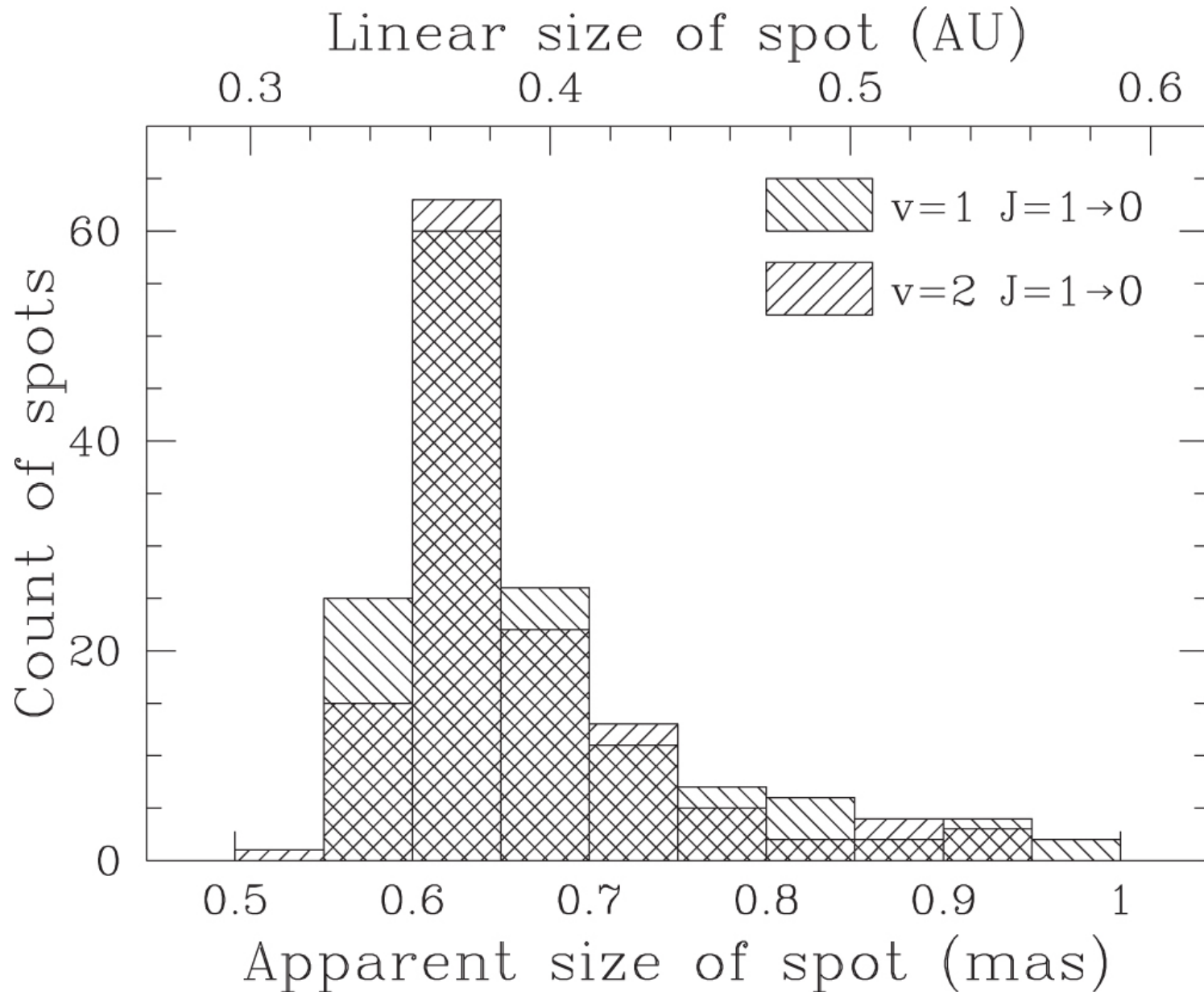
Figure 8. from SiO MASERS AROUND WX PSC MAPPED WITH THE KVN AND VERA ARRAY (KaVA) null 2016 APJ 822 3 doi:10.3847/0004-637X/822/1/3 https://dx.doi.org/10.3847/0004-637X/822/1/3 © 2016. The American Astronomical Society. All rights reserved.
