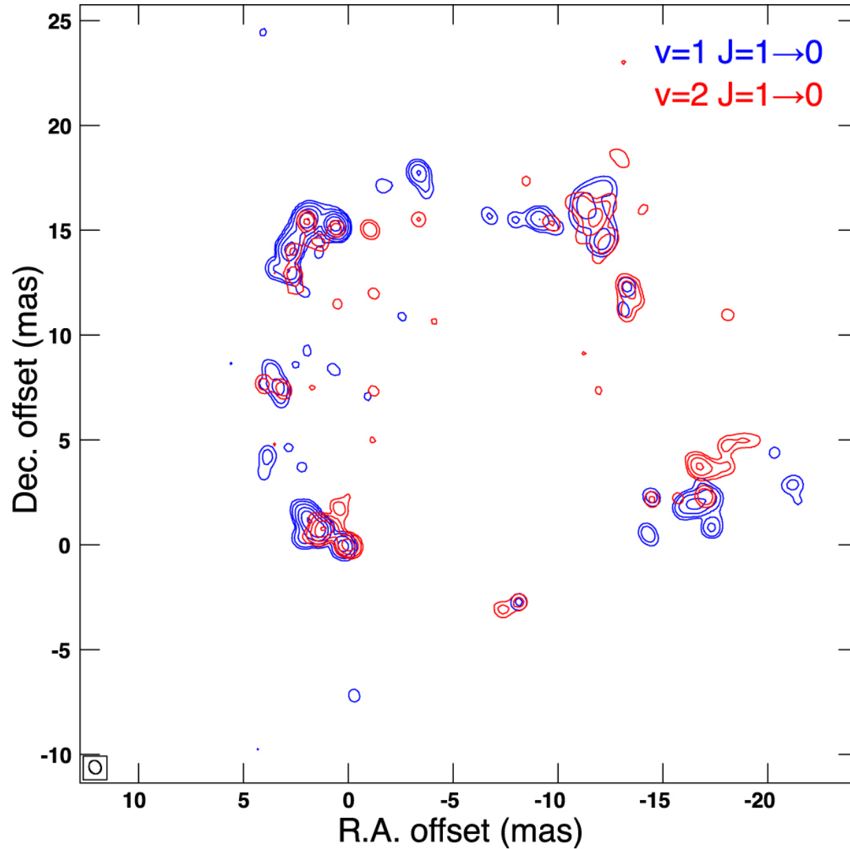
Figure 3. from SiO MASERS AROUND WX PSC MAPPED WITH THE KVN AND VERA ARRAY (KaVA) null 2016 APJ 822 3 doi:10.3847/0004-637X/822/1/3 https://dx.doi.org/10.3847/0004-637X/822/1/3 © 2016. The American Astronomical Society. All rights reserved.
