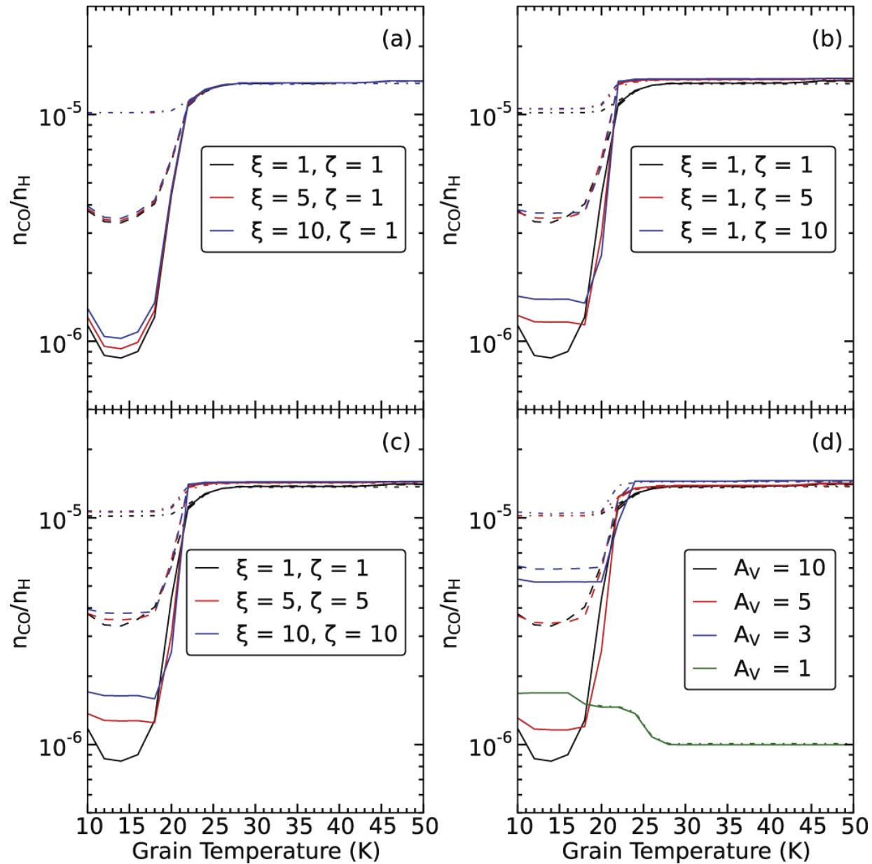
Figure 9. from SIMULATIONS OF THE CHEMISTRY IN THE SMALL MAGELLANIC CLOUD null 2016 APJ 822 105 doi:10.3847/0004-637X/822/2/105 https://dx.doi.org/10.3847/0004-637X/822/2/105 © 2016. The American Astronomical Society. All rights reserved.
