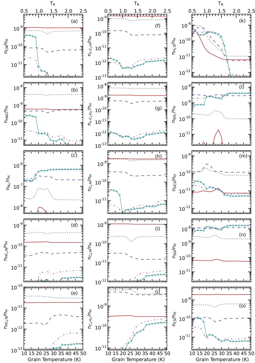
Figure 7. from SIMULATIONS OF THE CHEMISTRY IN THE SMALL MAGELLANIC CLOUD null 2016 APJ 822 105 doi:10.3847/0004-637X/822/2/105 https://dx.doi.org/10.3847/0004-637X/822/2/105 © 2016. The American Astronomical Society. All rights reserved.
