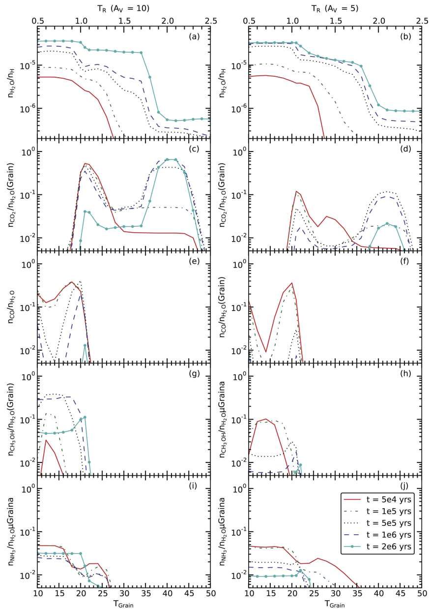
Figure 10. from SIMULATIONS OF THE CHEMISTRY IN THE SMALL MAGELLANIC CLOUD null 2016 APJ 822 105 doi:10.3847/0004-637X/822/2/105 https://dx.doi.org/10.3847/0004-637X/822/2/105 © 2016. The American Astronomical Society. All rights reserved.
