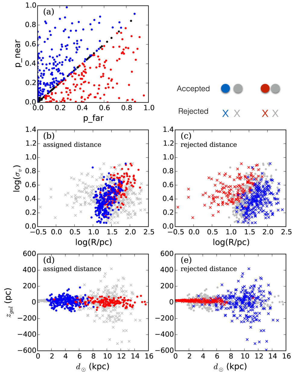
Figure 4. from A UNIFORM CATALOG OF MOLECULAR CLOUDS IN THE MILKY WAY null 2016 APJ 822 52 doi:10.3847/0004-637X/822/1/52 https://dx.doi.org/10.3847/0004-637X/822/1/52
