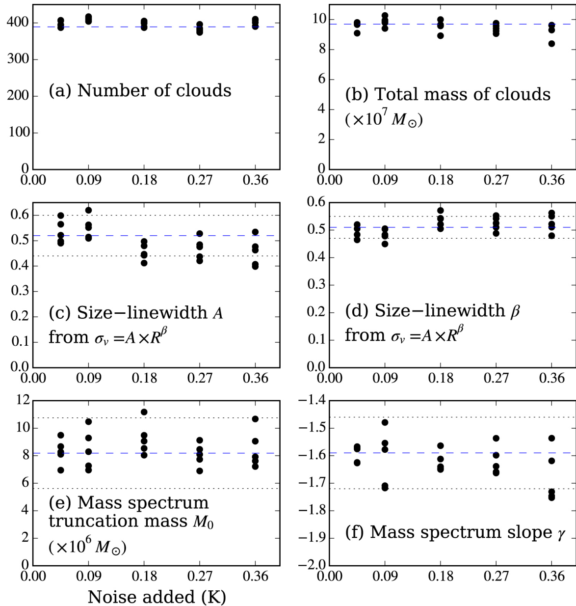
Figure 22. from A UNIFORM CATALOG OF MOLECULAR CLOUDS IN THE MILKY WAY null 2016 APJ 822 52 doi:10.3847/0004-637X/822/1/52 https://dx.doi.org/10.3847/0004-637X/822/1/52 © 2016. The American Astronomical Society. All rights reserved.
