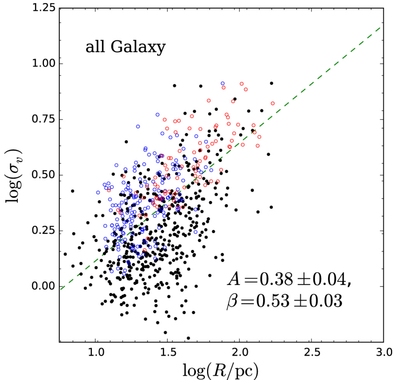
Figure 19. from A UNIFORM CATALOG OF MOLECULAR CLOUDS IN THE MILKY WAY null 2016 APJ 822 52 doi:10.3847/0004-637X/822/1/52 https://dx.doi.org/10.3847/0004-637X/822/1/52 © 2016. The American Astronomical Society. All rights reserved.
