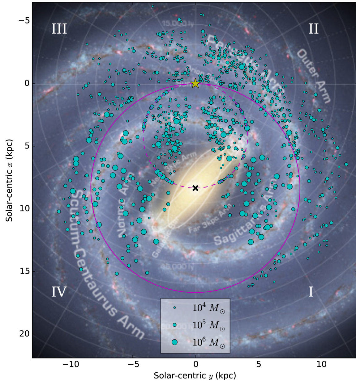
Figure 15. from A UNIFORM CATALOG OF MOLECULAR CLOUDS IN THE MILKY WAY null 2016 APJ 822 52 doi:10.3847/0004-637X/822/1/52 https://dx.doi.org/10.3847/0004-637X/822/1/52 © 2016. The American Astronomical Society. All rights reserved.
