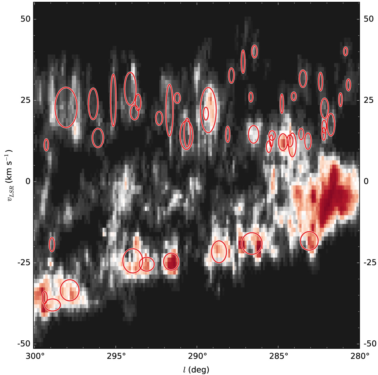
Figure 13. from A UNIFORM CATALOG OF MOLECULAR CLOUDS IN THE MILKY WAY null 2016 APJ 822 52 doi:10.3847/0004-637X/822/1/52 https://dx.doi.org/10.3847/0004-637X/822/1/52 © 2016. The American Astronomical Society. All rights reserved.
