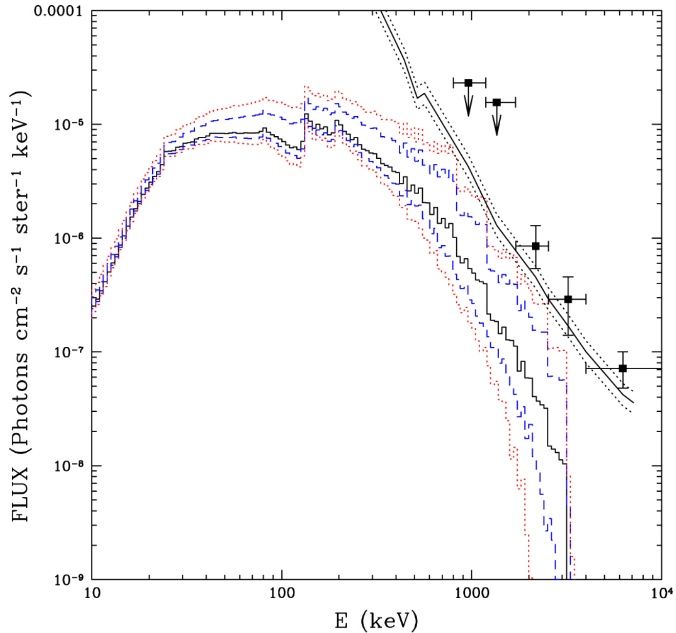
Figure 9. from THE ORIGIN OF THE COSMIC GAMMA-RAY BACKGROUND IN THE MeV RANGE null 2016 APJ 820 142 doi:10.3847/0004-637X/820/2/142 https://dx.doi.org/10.3847/0004-637X/820/2/142 © 2016. The American Astronomical Society. All rights reserved.
