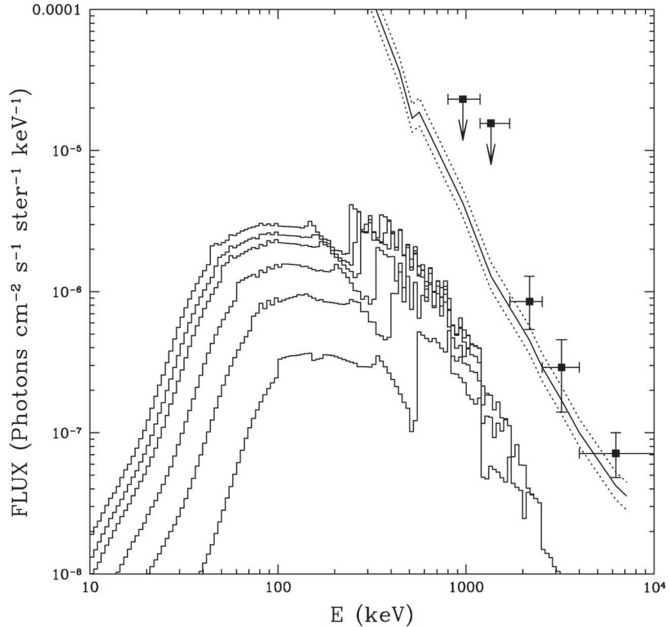
Figure 7. from THE ORIGIN OF THE COSMIC GAMMA-RAY BACKGROUND IN THE MeV RANGE null 2016 APJ 820 142 doi:10.3847/0004-637X/820/2/142 https://dx.doi.org/10.3847/0004-637X/820/2/142 © 2016. The American Astronomical Society. All rights reserved.
