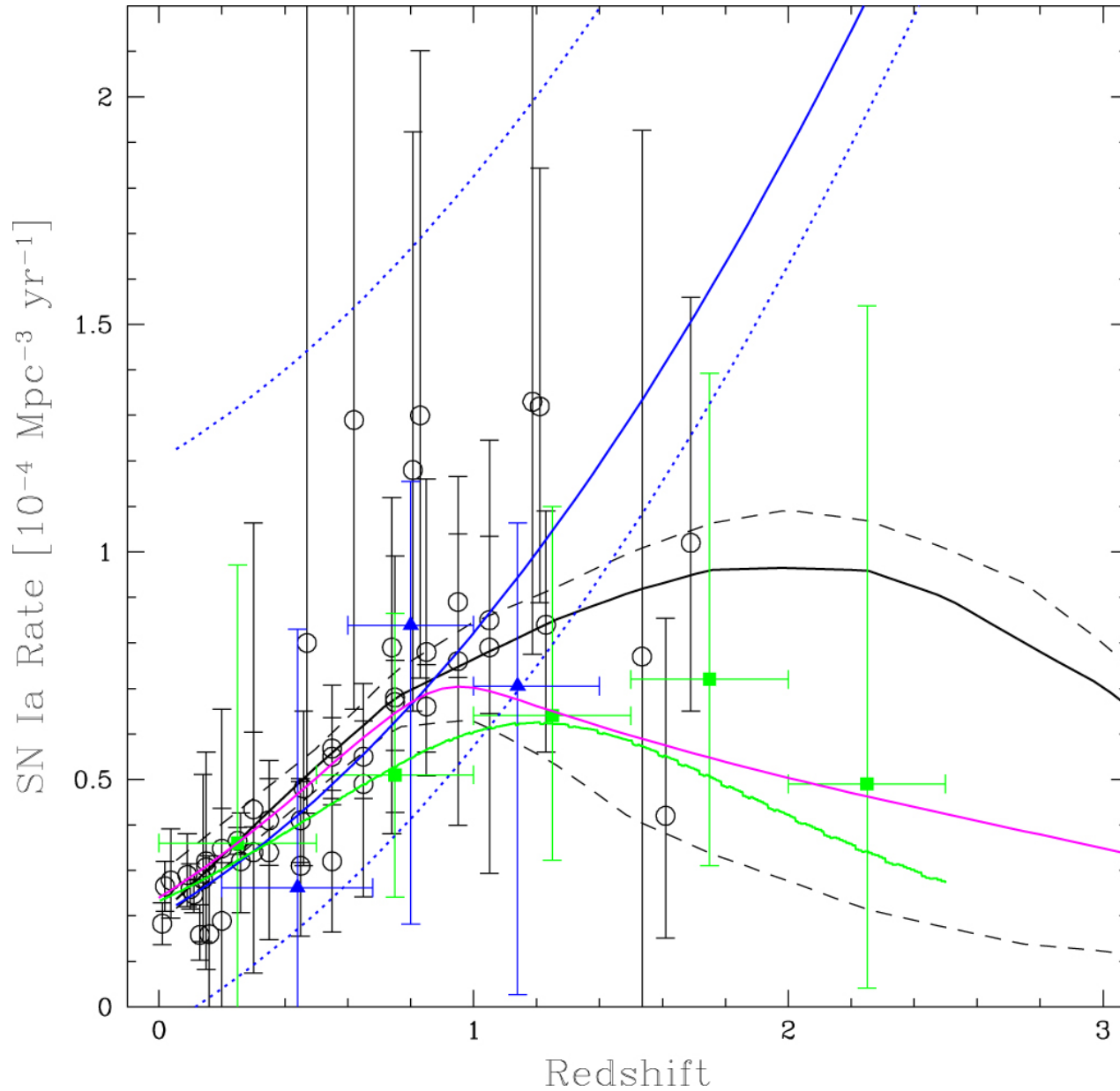
Figure 6. from THE ORIGIN OF THE COSMIC GAMMA-RAY BACKGROUND IN THE MeV RANGE null 2016 APJ 820 142 doi:10.3847/0004-637X/820/2/142 https://dx.doi.org/10.3847/0004-637X/820/2/142 © 2016. The American Astronomical Society. All rights reserved.
