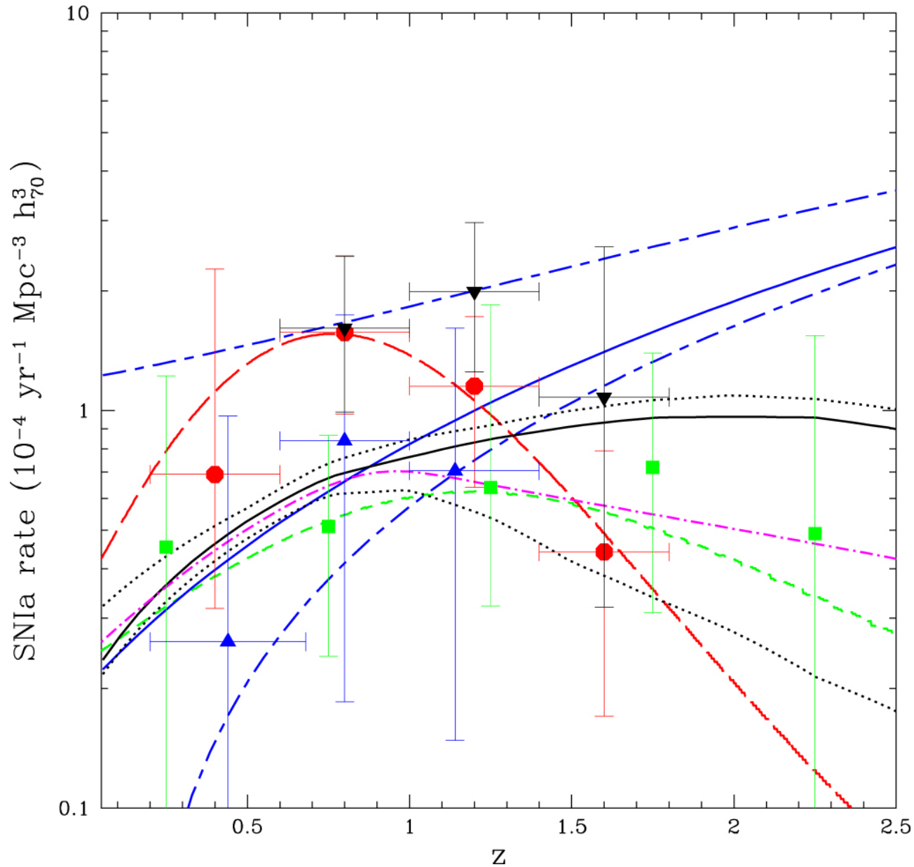
Figure 5. from THE ORIGIN OF THE COSMIC GAMMA-RAY BACKGROUND IN THE MeV RANGE null 2016 APJ 820 142 doi:10.3847/0004-637X/820/2/142 https://dx.doi.org/10.3847/0004-637X/820/2/142 © 2016. The American Astronomical Society. All rights reserved.
