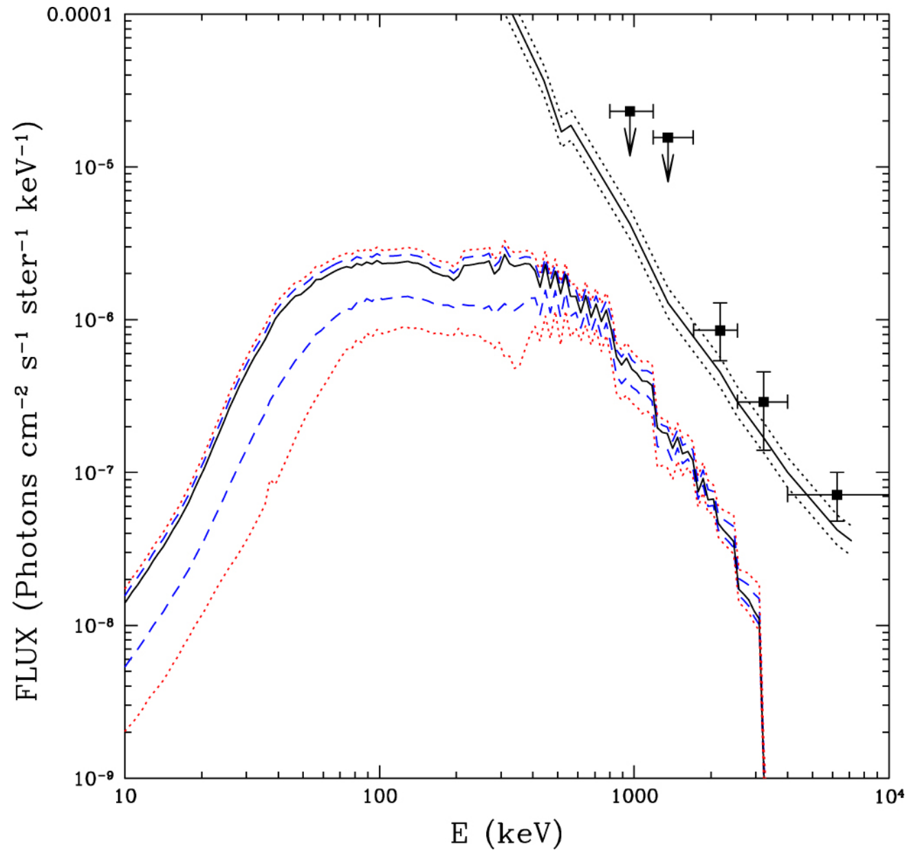
Figure 10. from THE ORIGIN OF THE COSMIC GAMMA-RAY BACKGROUND IN THE MeV RANGE null 2016 APJ 820 142 doi:10.3847/0004-637X/820/2/142 https://dx.doi.org/10.3847/0004-637X/820/2/142 © 2016. The American Astronomical Society. All rights reserved.
