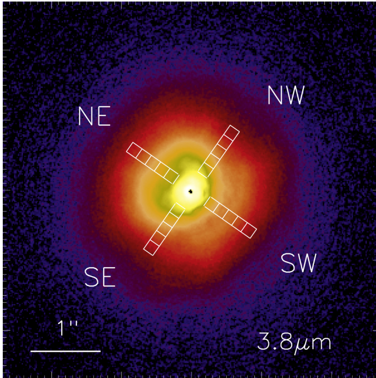
Figure 2. from WATER ICE AT THE SURFACE OF THE HD 100546 DISK null 2016 APJ 821 2 doi:10.3847/0004-637X/821/1/2 https://dx.doi.org/10.3847/0004-637X/821/1/2 © 2016. The American Astronomical Society. All rights reserved.
