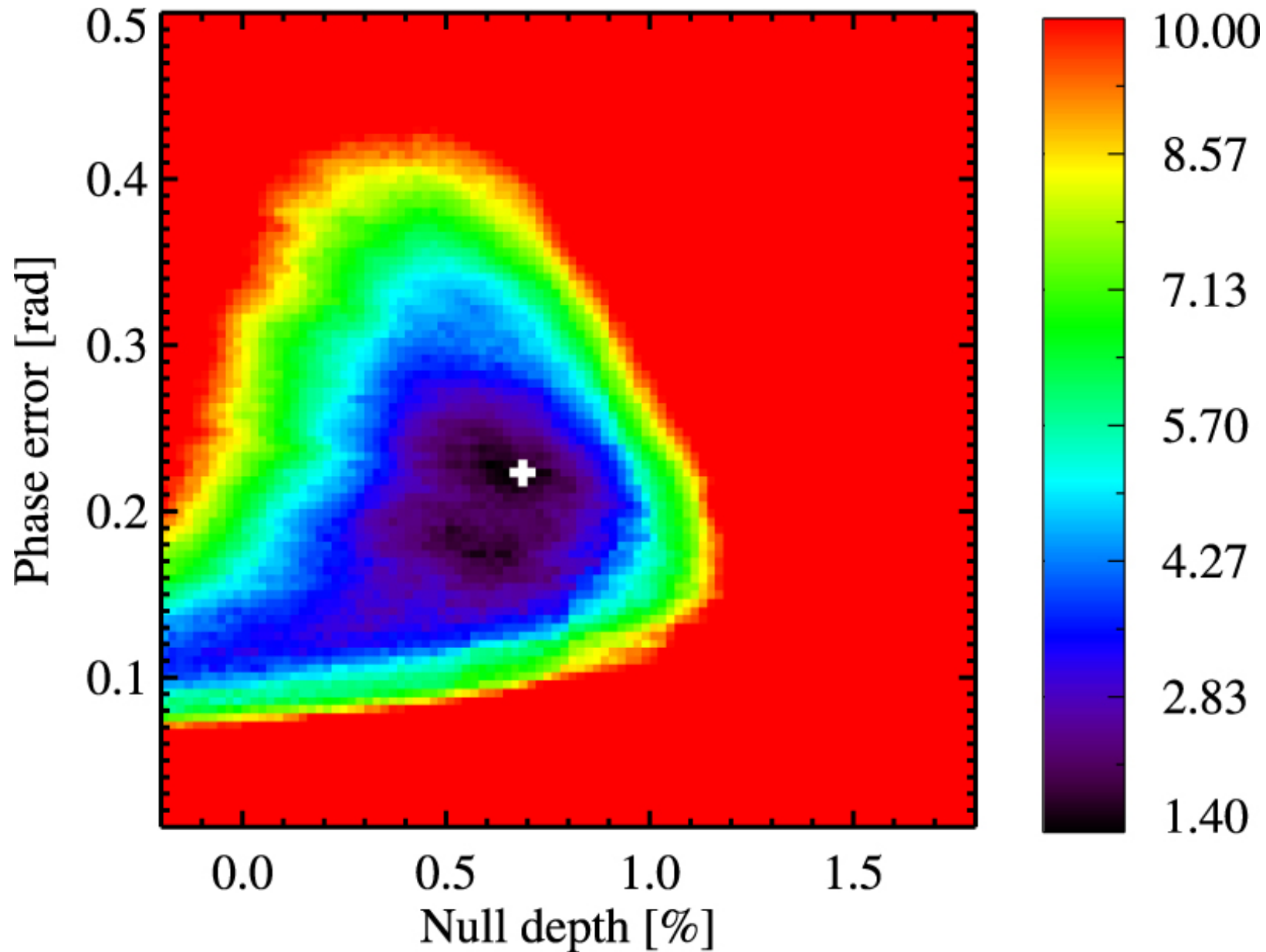
Figure 9. from NULLING DATA REDUCTION AND ON-SKY PERFORMANCE OF THE LARGE BINOCULAR TELESCOPE INTERFEROMETER null 2016 APJ 824 66 doi:10.3847/0004-637X/824/2/66 https://dx.doi.org/10.3847/0004-637X/824/2/66 © 2016. The American Astronomical Society. All rights reserved.
