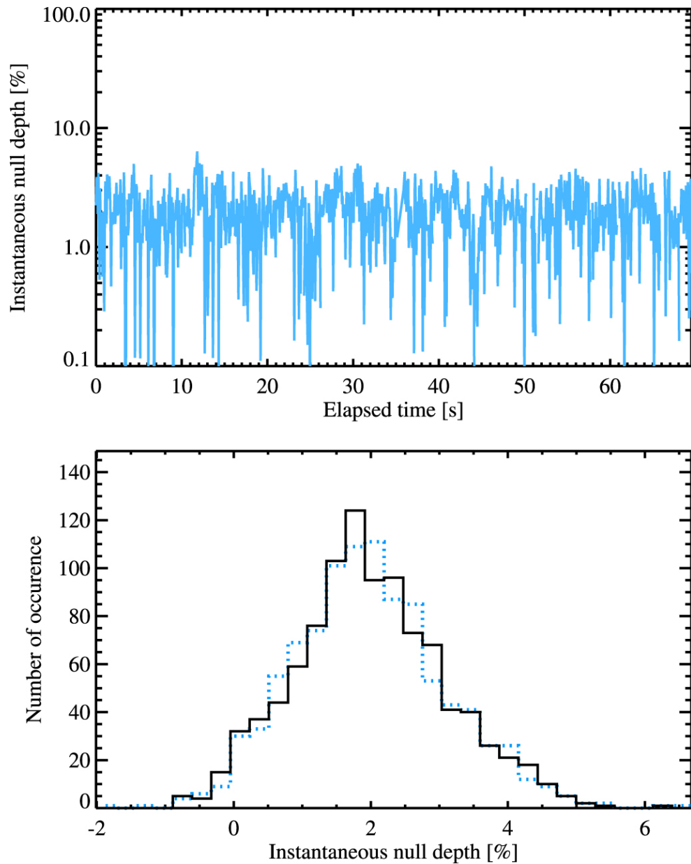
Figure 8. from NULLING DATA REDUCTION AND ON-SKY PERFORMANCE OF THE LARGE BINOCULAR TELESCOPE INTERFEROMETER null 2016 APJ 824 66 doi:10.3847/0004-637X/824/2/66 https://dx.doi.org/10.3847/0004-637X/824/2/66 © 2016. The American Astronomical Society. All rights reserved.
