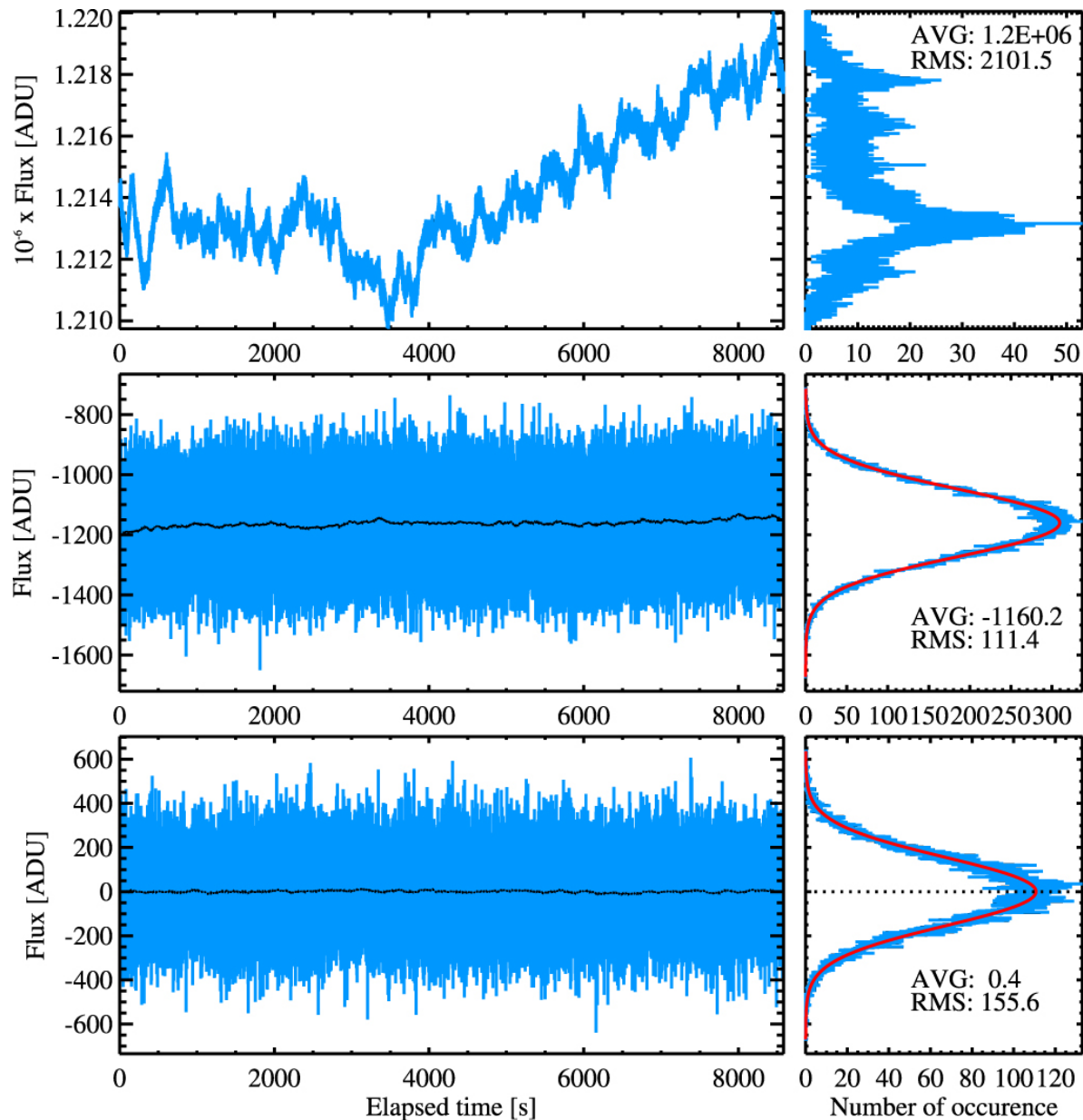
Figure 7. from NULLING DATA REDUCTION AND ON-SKY PERFORMANCE OF THE LARGE BINOCULAR TELESCOPE INTERFEROMETER null 2016 APJ 824 66 doi:10.3847/0004-637X/824/2/66 https://dx.doi.org/10.3847/0004-637X/824/2/66
