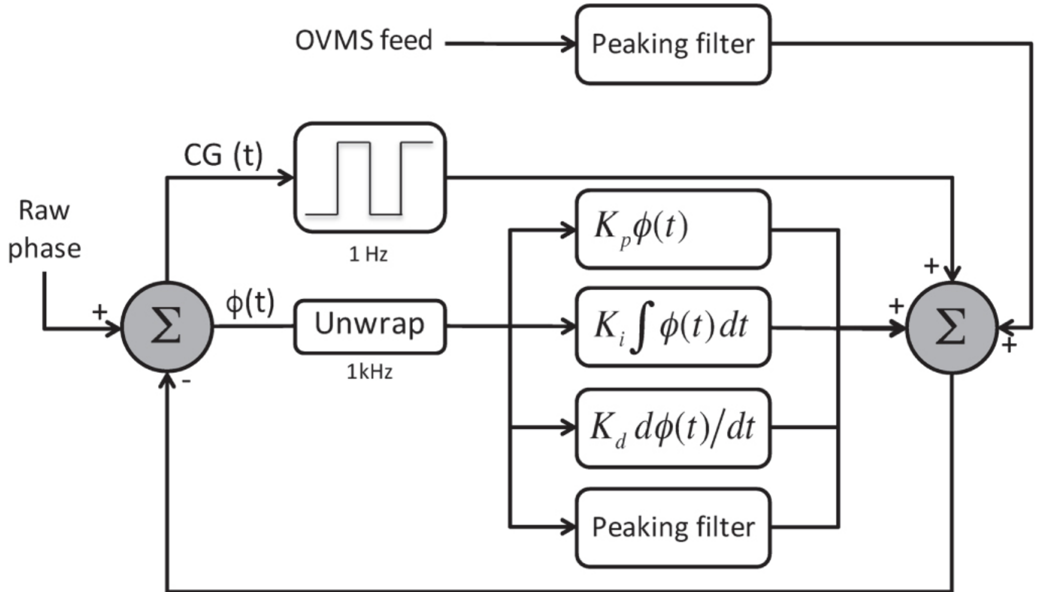
Figure 5. from NULLING DATA REDUCTION AND ON-SKY PERFORMANCE OF THE LARGE BINOCULAR TELESCOPE INTERFEROMETER null 2016 APJ 824 66 doi:10.3847/0004-637X/824/2/66 https://dx.doi.org/10.3847/0004-637X/824/2/66 © 2016. The American Astronomical Society. All rights reserved.
