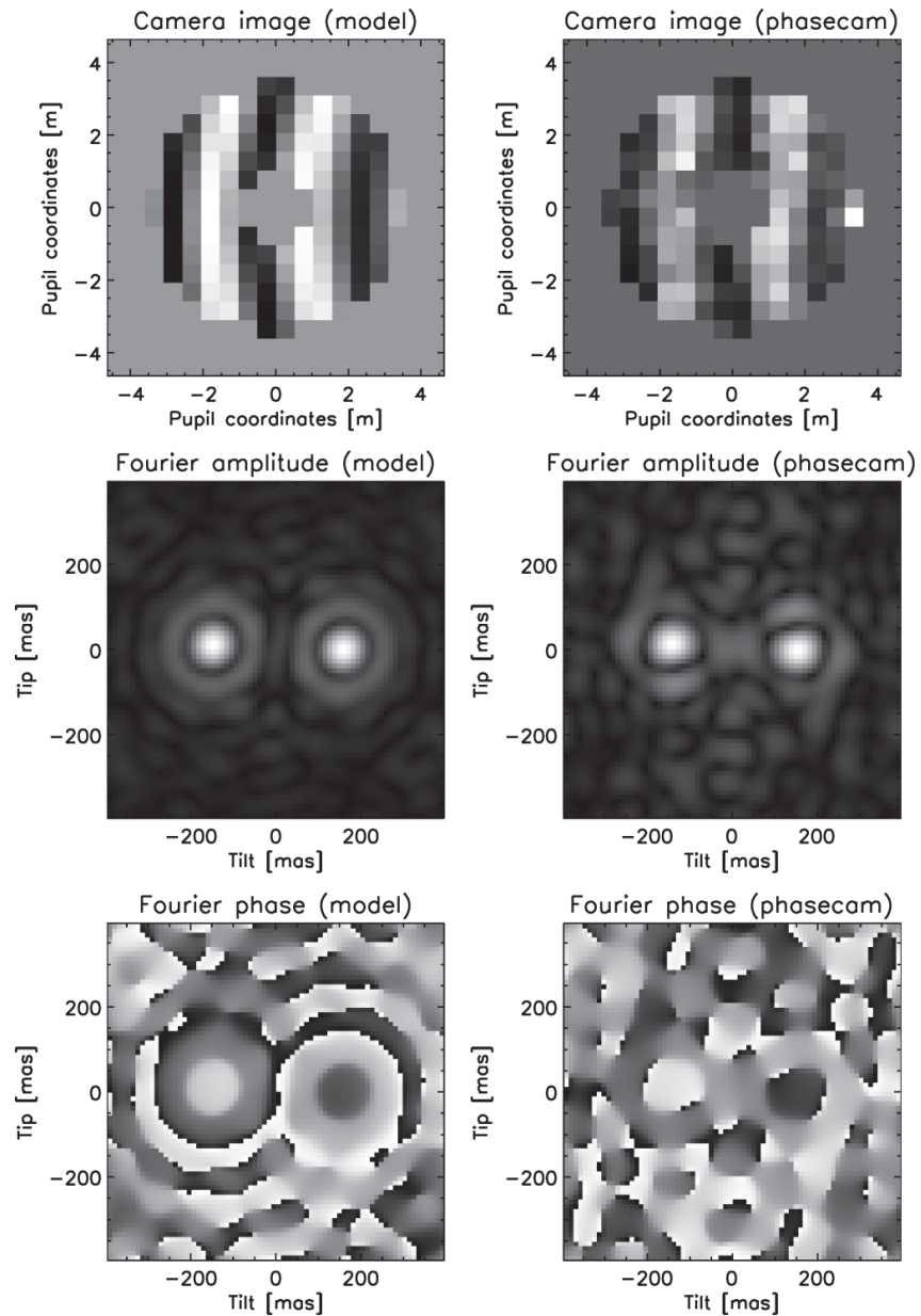
Figure 4. from NULLING DATA REDUCTION AND ON-SKY PERFORMANCE OF THE LARGE BINOCULAR TELESCOPE INTERFEROMETER null 2016 APJ 824 66 doi:10.3847/0004-637X/824/2/66 https://dx.doi.org/10.3847/0004-637X/824/2/66
