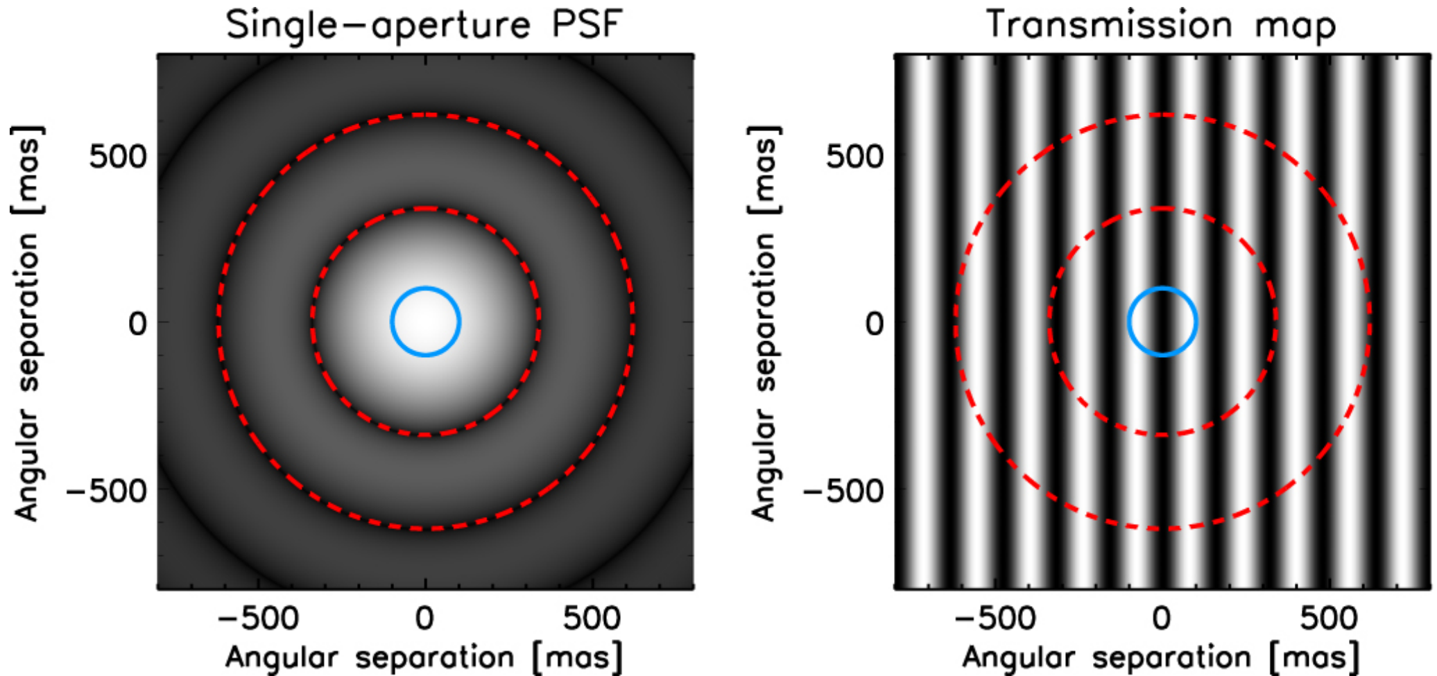
Figure 3. from NULLING DATA REDUCTION AND ON-SKY PERFORMANCE OF THE LARGE BINOCULAR TELESCOPE INTERFEROMETER null 2016 APJ 824 66 doi:10.3847/0004-637X/824/2/66 https://dx.doi.org/10.3847/0004-637X/824/2/66 © 2016. The American Astronomical Society. All rights reserved.
