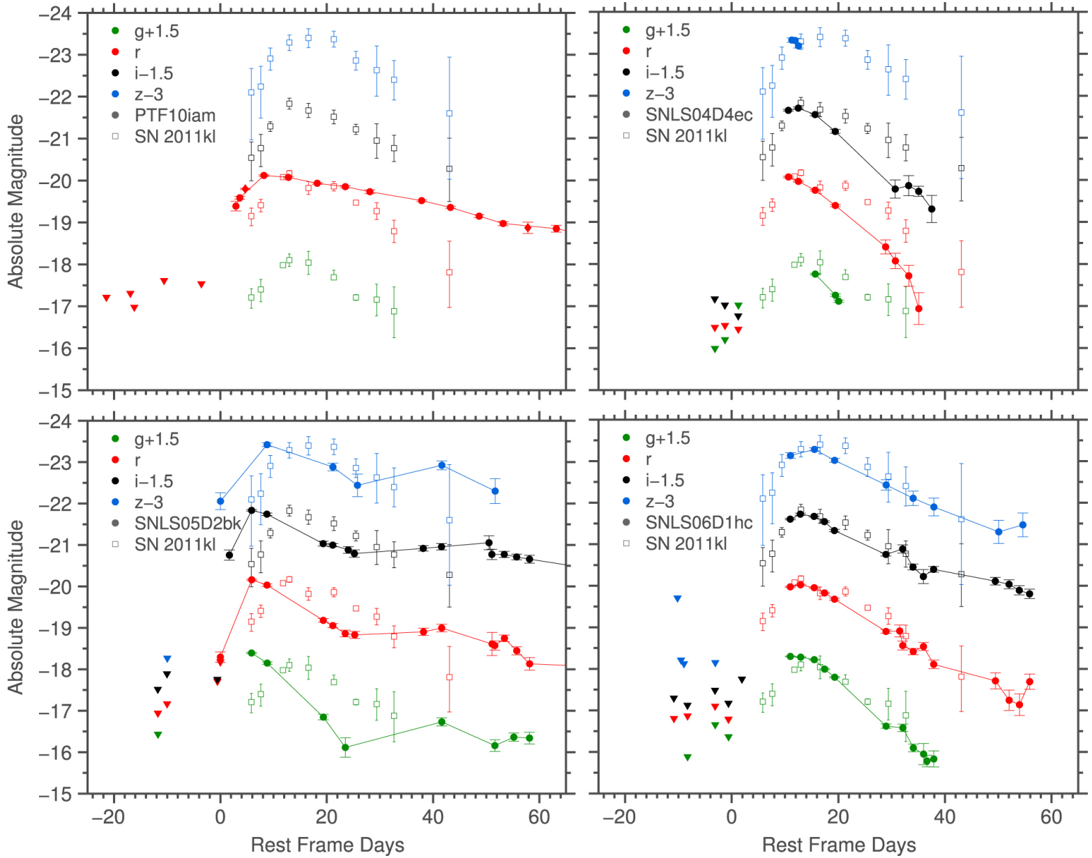
Figure 9. from RAPIDLY RISING TRANSIENTS IN THE SUPERNOVA—SUPERLUMINOUS SUPERNOVA GAP null 2016 APJ 819 35 doi:10.3847/0004-637X/819/1/35 https://dx.doi.org/10.3847/0004-637X/819/1/35 © 2016. The American Astronomical Society. All rights reserved.
