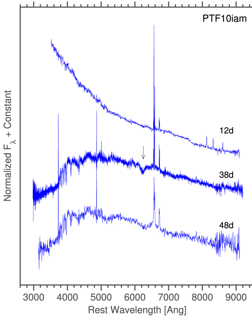
Figure 5. from RAPIDLY RISING TRANSIENTS IN THE SUPERNOVA—SUPERLUMINOUS SUPERNOVA GAP null 2016 APJ 819 35 doi:10.3847/0004-637X/819/1/35 https://dx.doi.org/10.3847/0004-637X/819/1/35 © 2016. The American Astronomical Society. All rights reserved.
