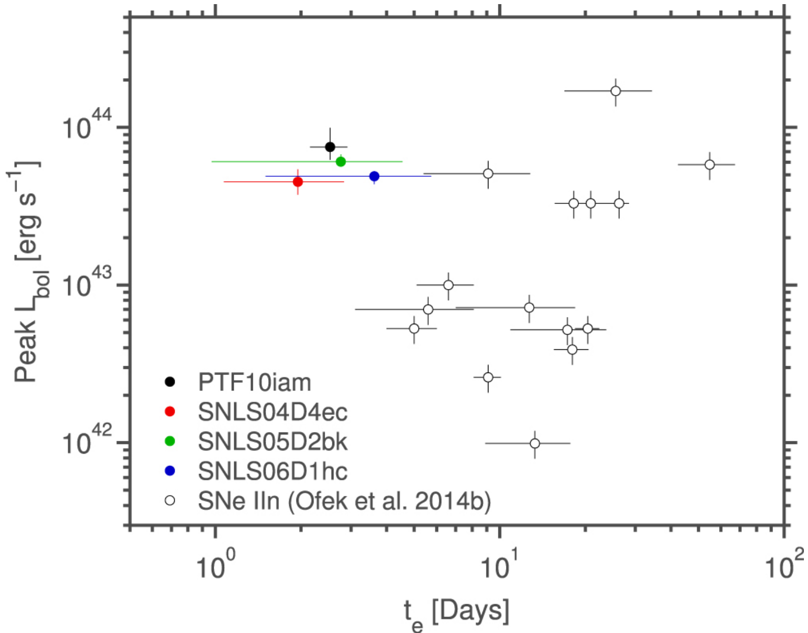
Figure 17. from RAPIDLY RISING TRANSIENTS IN THE SUPERNOVA—SUPERLUMINOUS SUPERNOVA GAP null 2016 APJ 819 35 doi:10.3847/0004-637X/819/1/35 https://dx.doi.org/10.3847/0004-637X/819/1/35 © 2016. The American Astronomical Society. All rights reserved.
