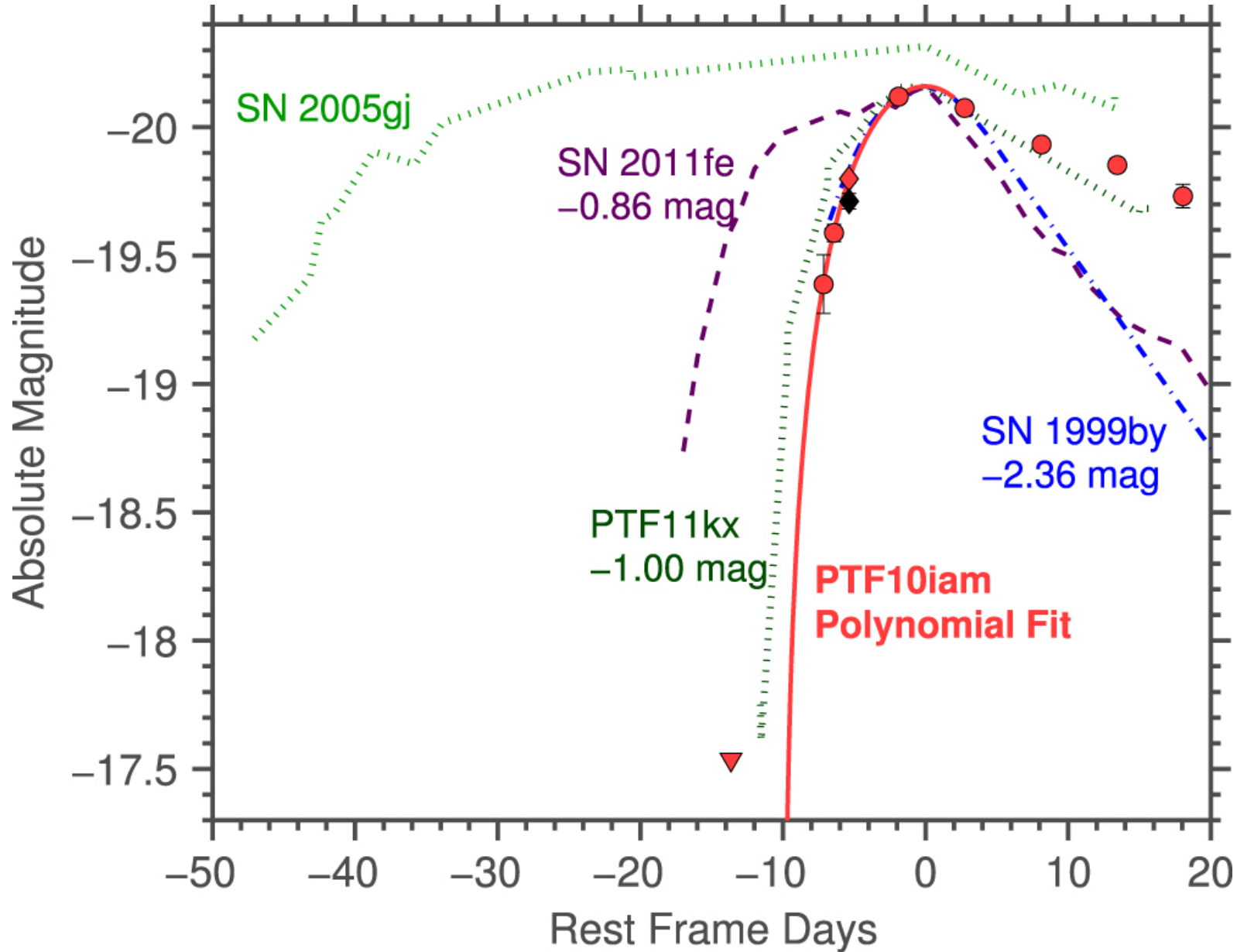
Figure 14. from RAPIDLY RISING TRANSIENTS IN THE SUPERNOVA—SUPERLUMINOUS SUPERNOVA GAP null 2016 APJ 819 35 doi:10.3847/0004-637X/819/1/35 https://dx.doi.org/10.3847/0004-637X/819/1/35 © 2016. The American Astronomical Society. All rights reserved.
