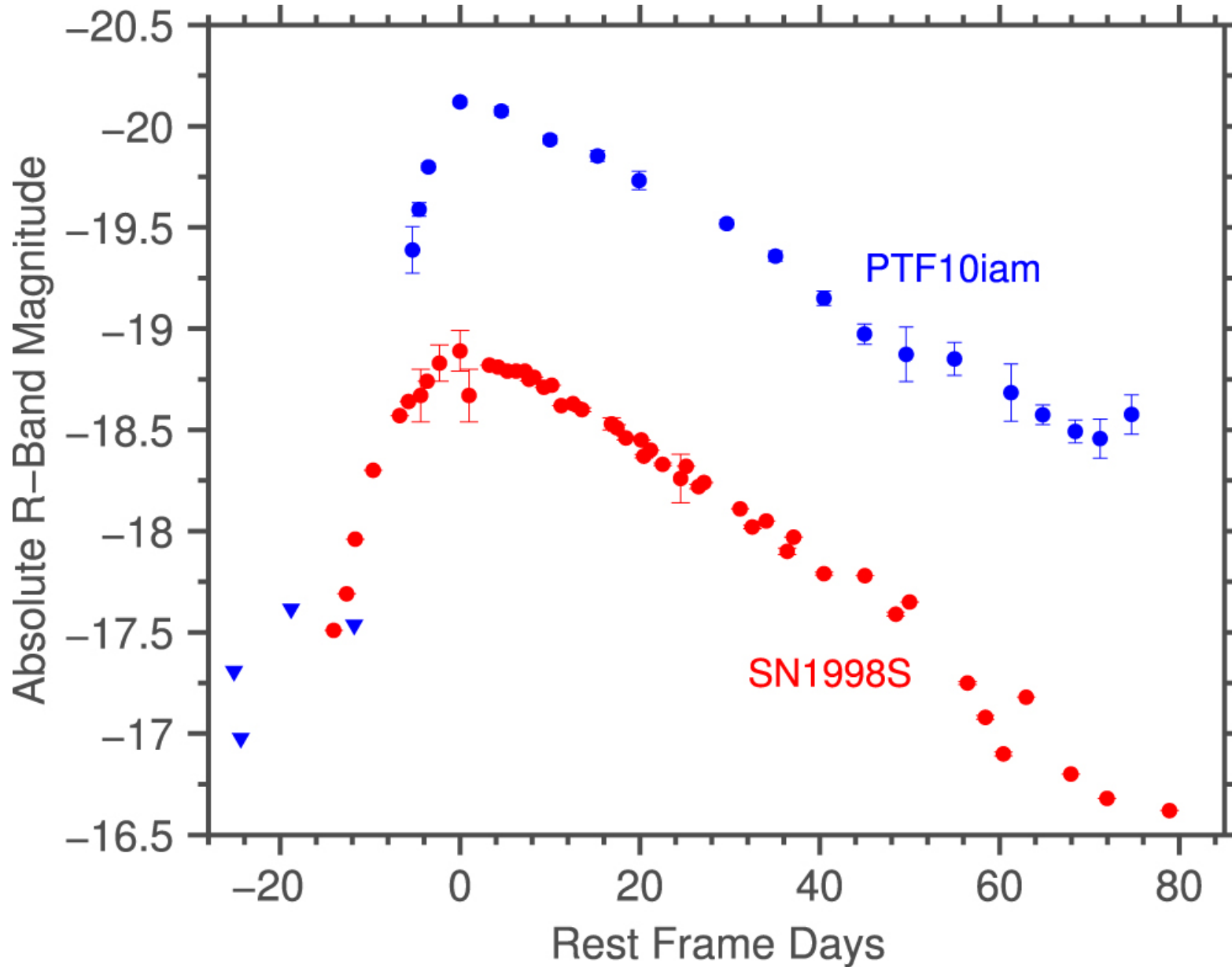
Figure 13. from RAPIDLY RISING TRANSIENTS IN THE SUPERNOVA—SUPERLUMINOUS SUPERNOVA GAP null 2016 APJ 819 35 doi:10.3847/0004-637X/819/1/35 https://dx.doi.org/10.3847/0004-637X/819/1/35 © 2016. The American Astronomical Society. All rights reserved.
