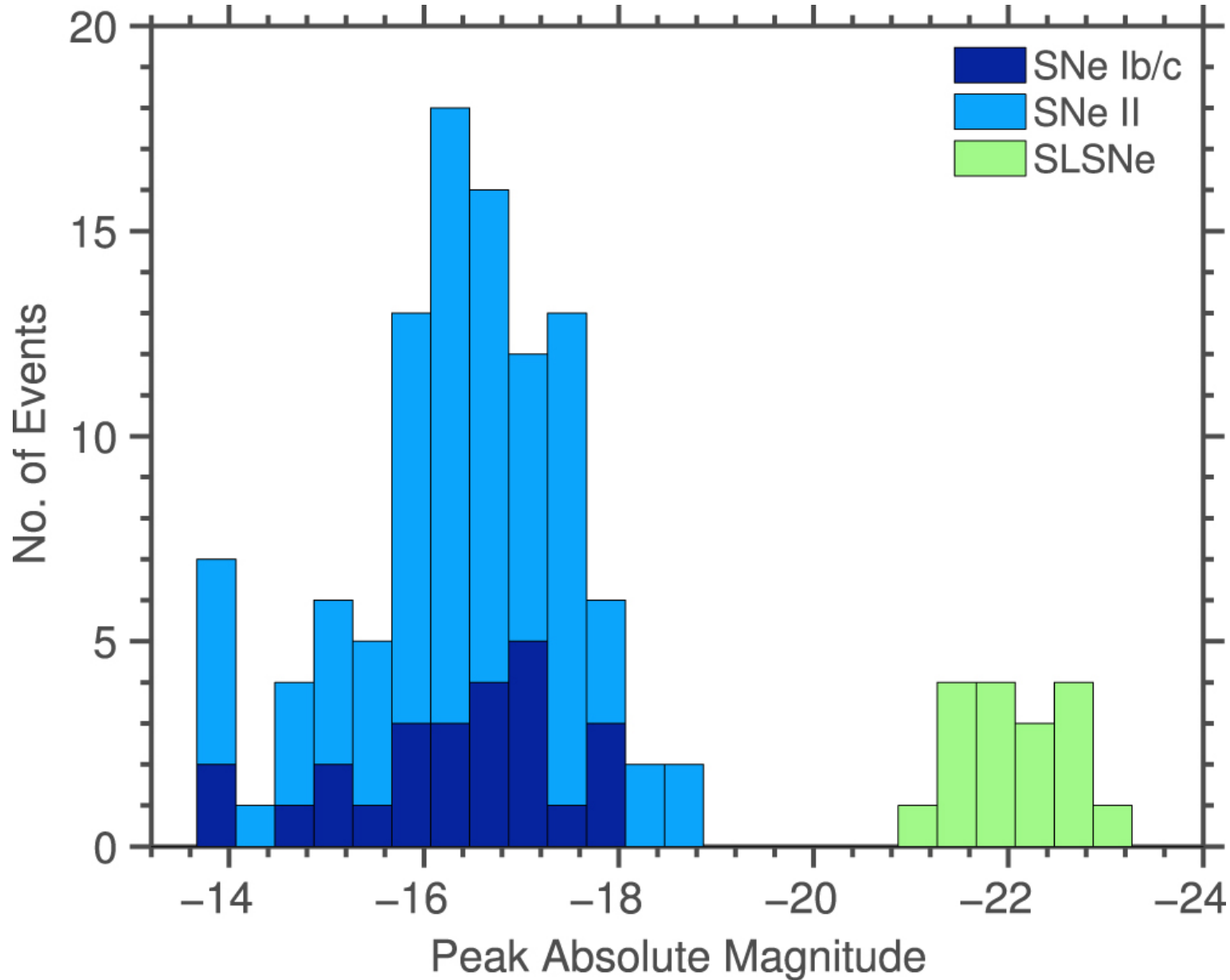
Figure 1. from RAPIDLY RISING TRANSIENTS IN THE SUPERNOVA—SUPERLUMINOUS SUPERNOVA GAP null 2016 APJ 819 35 doi:10.3847/0004-637X/819/1/35 https://dx.doi.org/10.3847/0004-637X/819/1/35 © 2016. The American Astronomical Society. All rights reserved.
