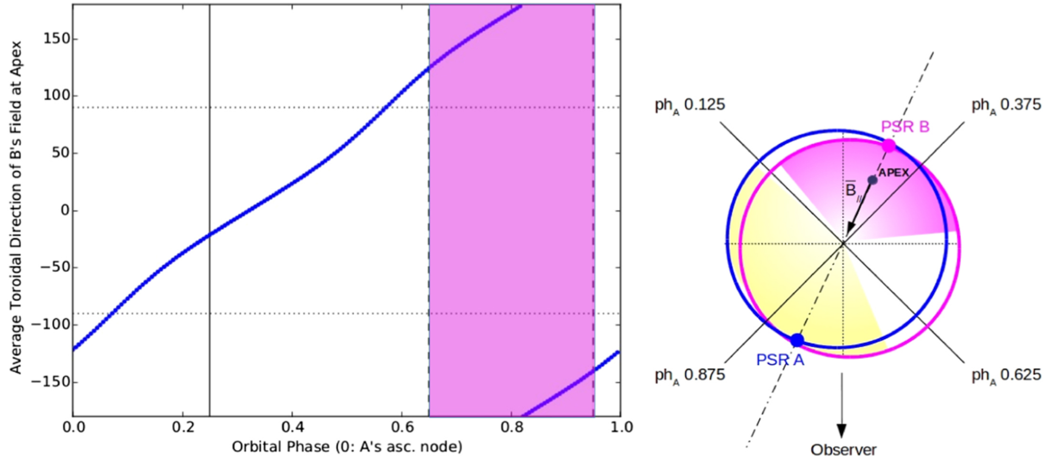
Figure 6. from LONG-TERM STUDY OF THE DOUBLE PULSAR J0737–3039 WITH XMM-NEWTON: PULSAR TIMING null 2016 APJ 824 87 doi:10.3847/0004-637X/824/2/87 https://dx.doi.org/10.3847/0004-637X/824/2/87 © 2016. The American Astronomical Society. All rights reserved.
