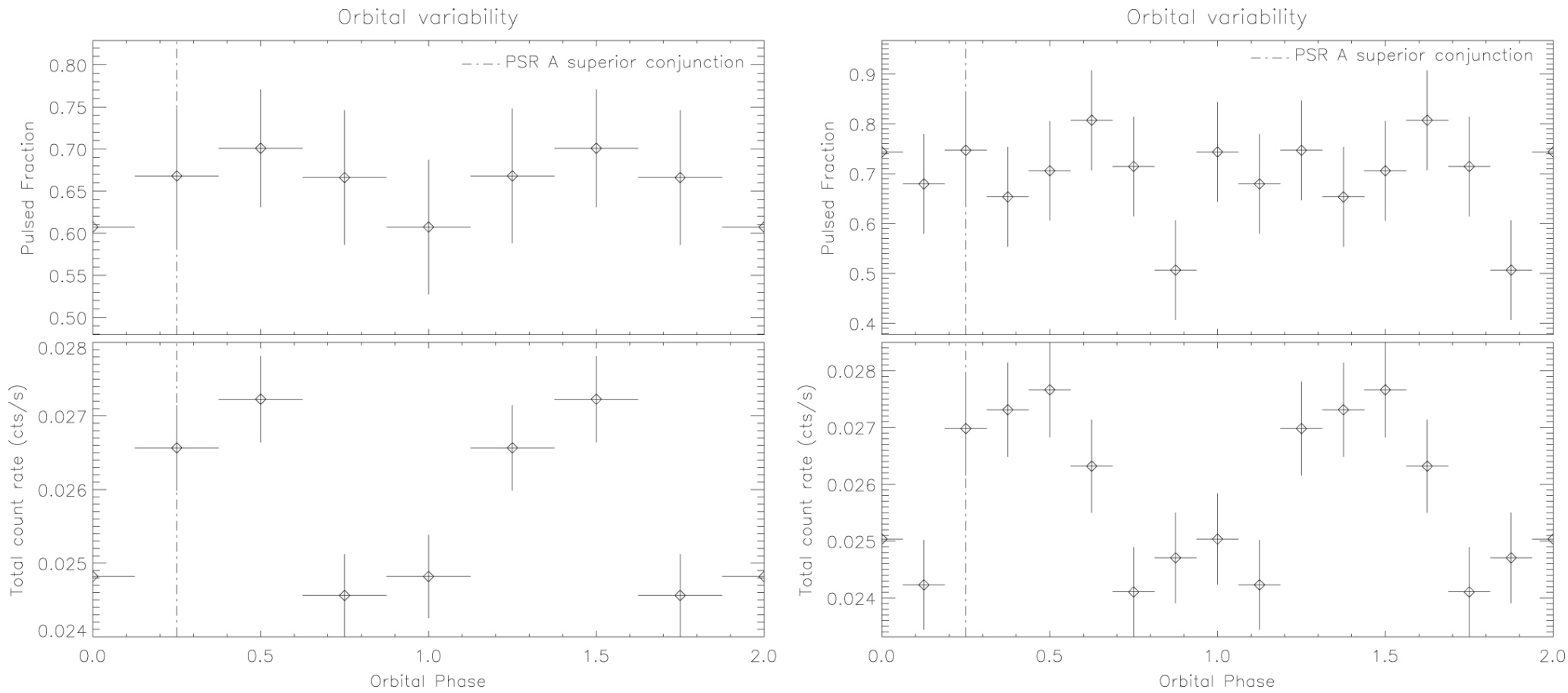
Figure 5. from LONG-TERM STUDY OF THE DOUBLE PULSAR J0737–3039 WITH XMM-NEWTON: PULSAR TIMING null 2016 APJ 824 87 doi:10.3847/0004-637X/824/2/87 https://dx.doi.org/10.3847/0004-637X/824/2/87 © 2016. The American Astronomical Society. All rights reserved.
