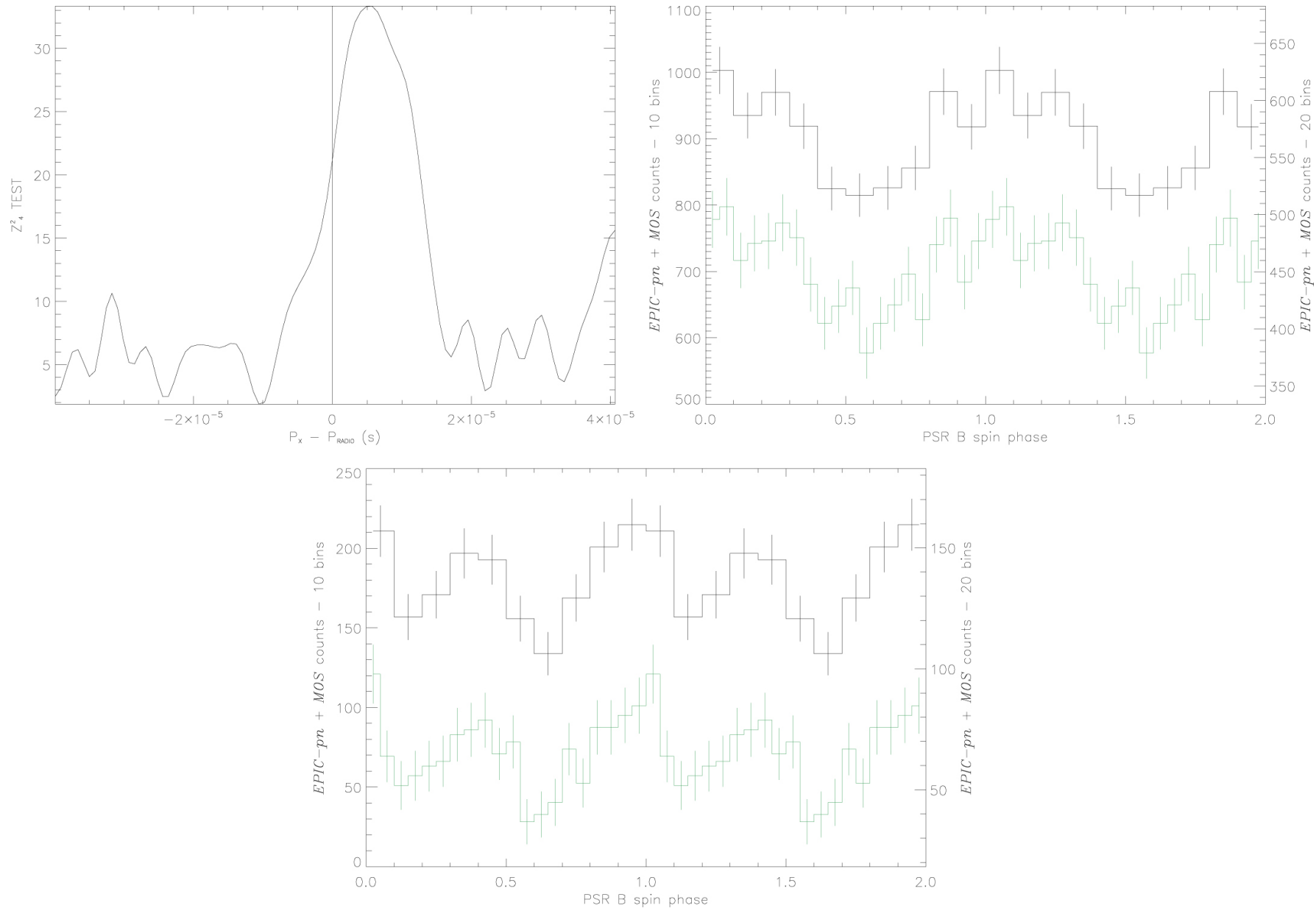
Figure 3. from LONG-TERM STUDY OF THE DOUBLE PULSAR J0737–3039 WITH XMM-NEWTON: PULSAR TIMING null 2016 APJ 824 87 doi:10.3847/0004-637X/824/2/87 https://dx.doi.org/10.3847/0004-637X/824/2/87 © 2016. The American Astronomical Society. All rights reserved.
