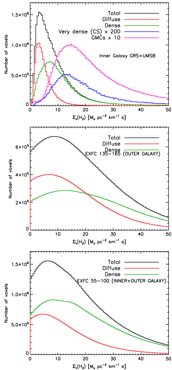
Figure 8. from DISTRIBUTION AND MASS OF DIFFUSE AND DENSE CO GAS IN THE MILKY WAY null 2016 APJ 818 144 doi:10.3847/0004-637X/818/2/144 https://dx.doi.org/10.3847/0004-637X/818/2/144 © 2016. The American Astronomical Society. All rights reserved.
