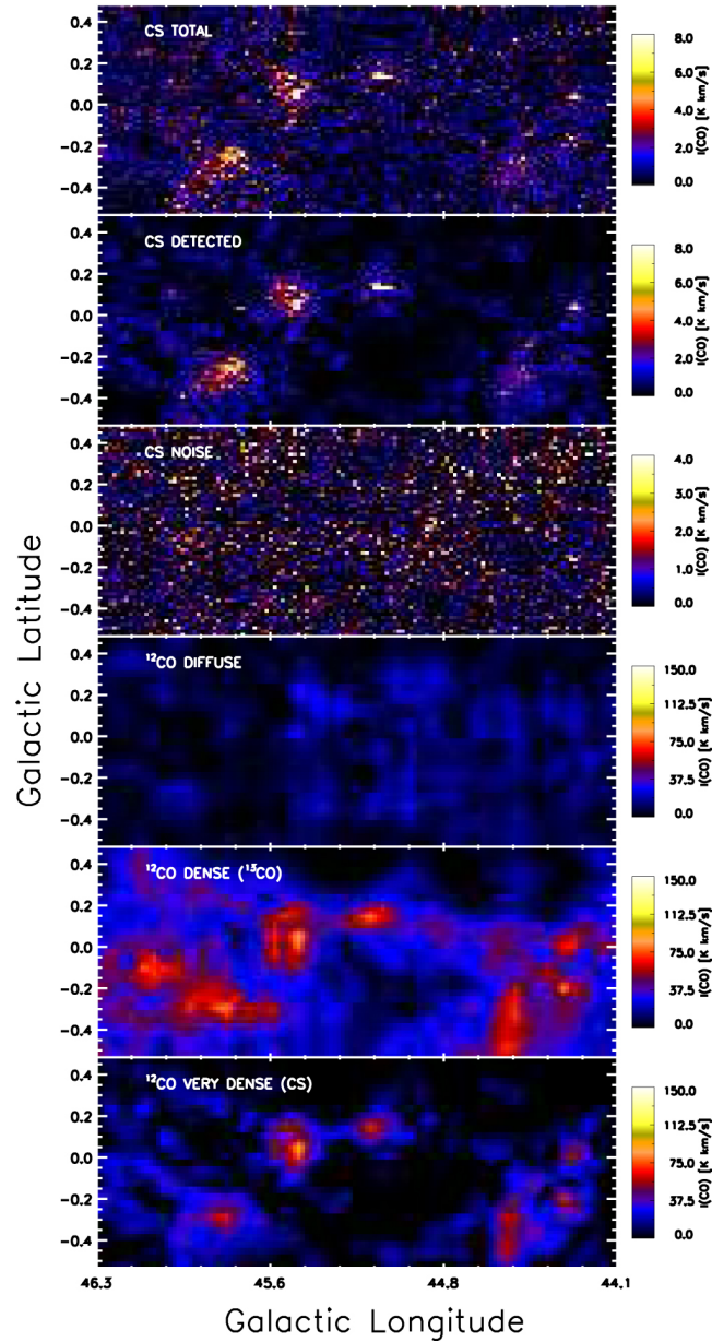
Figure 4. from DISTRIBUTION AND MASS OF DIFFUSE AND DENSE CO GAS IN THE MILKY WAY null 2016 APJ 818 144 doi:10.3847/0004-637X/818/2/144 https://dx.doi.org/10.3847/0004-637X/818/2/144 © 2016. The American Astronomical Society. All rights reserved.
