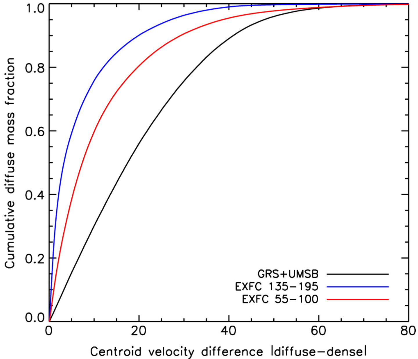
Figure 17. from DISTRIBUTION AND MASS OF DIFFUSE AND DENSE CO GAS IN THE MILKY WAY null 2016 APJ 818 144 doi:10.3847/0004-637X/818/2/144 https://dx.doi.org/10.3847/0004-637X/818/2/144 © 2016. The American Astronomical Society. All rights reserved.
