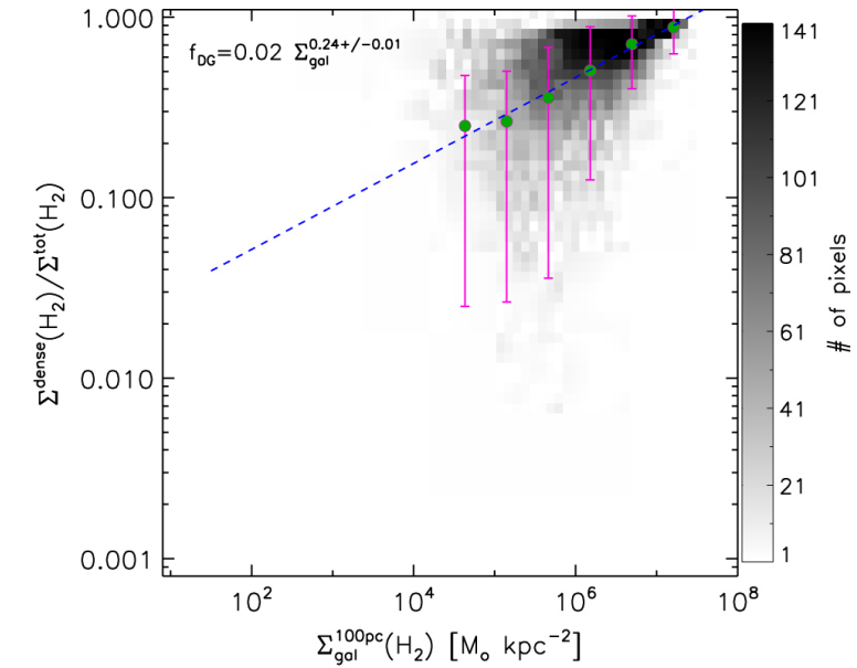
Figure 14. from DISTRIBUTION AND MASS OF DIFFUSE AND DENSE CO GAS IN THE MILKY WAY null 2016 APJ 818 144 doi:10.3847/0004-637X/818/2/144 https://dx.doi.org/10.3847/0004-637X/818/2/144
