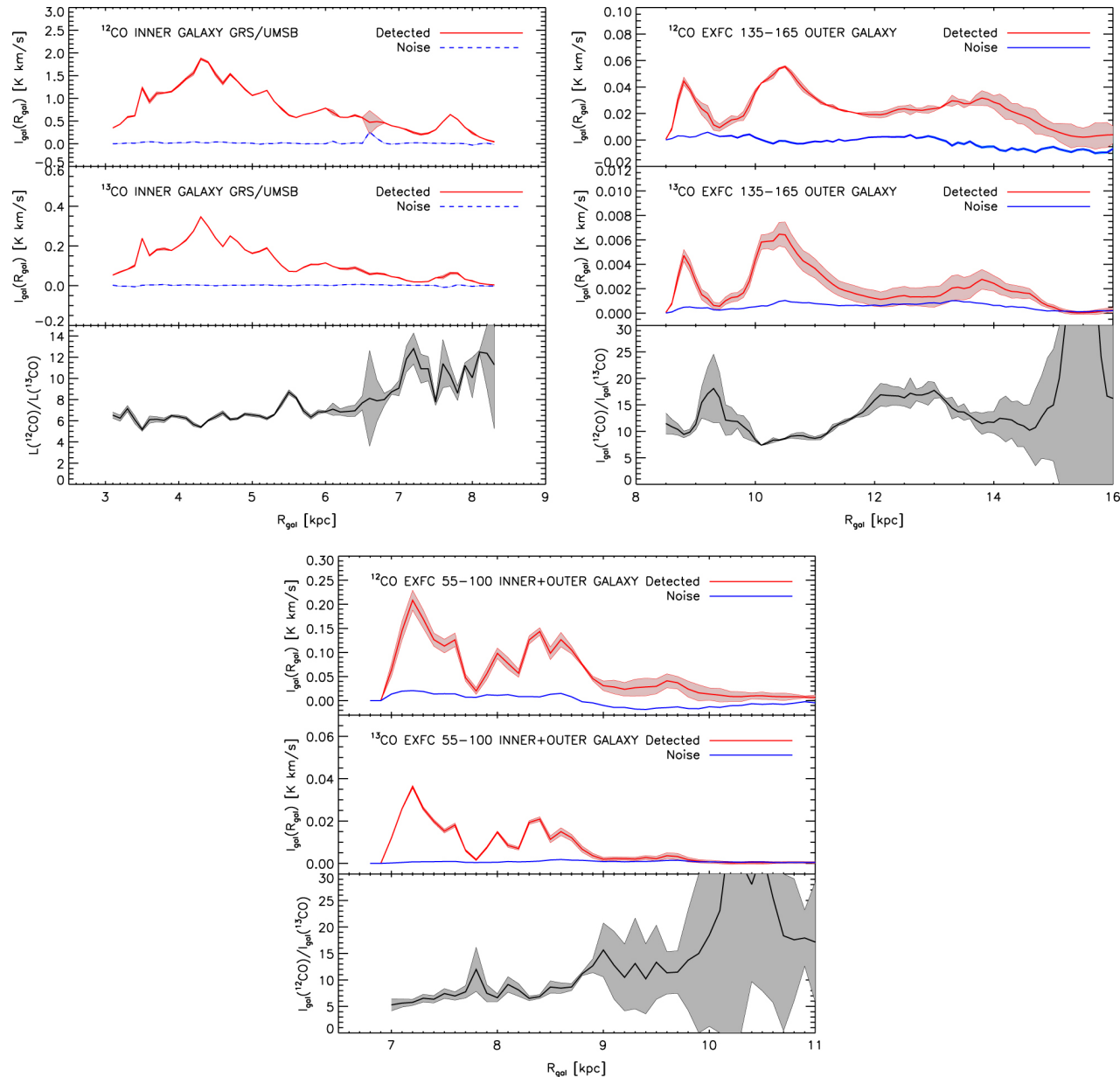
Figure 10. from DISTRIBUTION AND MASS OF DIFFUSE AND DENSE CO GAS IN THE MILKY WAY null 2016 APJ 818 144 doi:10.3847/0004-637X/818/2/144 https://dx.doi.org/10.3847/0004-637X/818/2/144
