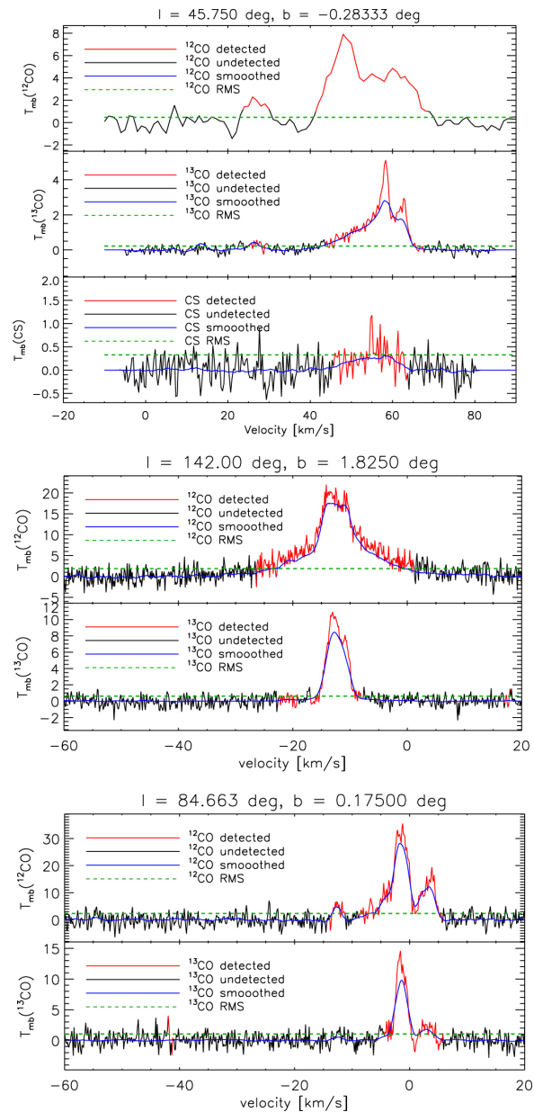
Figure 1. from DISTRIBUTION AND MASS OF DIFFUSE AND DENSE CO GAS IN THE MILKY WAY null 2016 APJ 818 144 doi:10.3847/0004-637X/818/2/144 https://dx.doi.org/10.3847/0004-637X/818/2/144 © 2016. The American Astronomical Society. All rights reserved.
