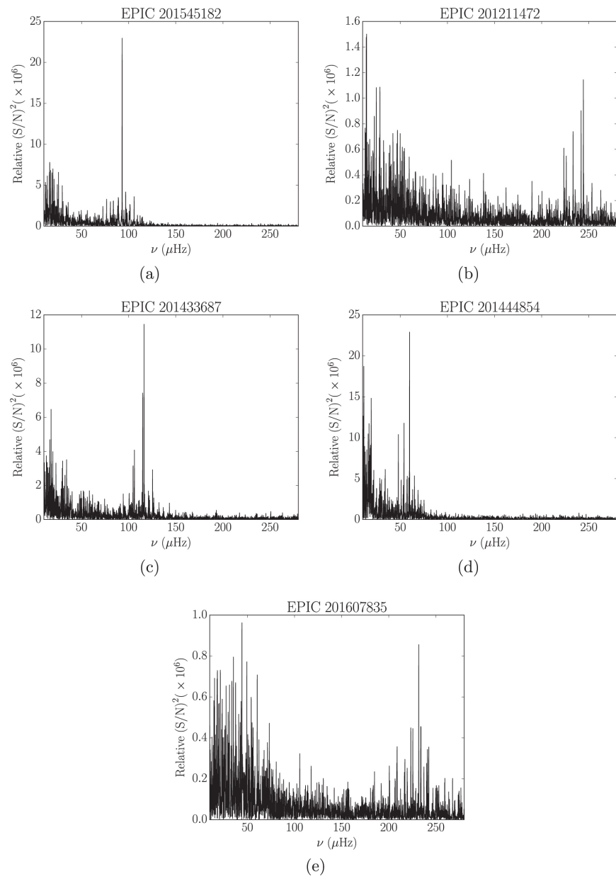
Figure 2. from SYSTEMATICS-INSENSITIVE PERIODIC SIGNAL SEARCH WITH K2 null 2016 APJ 818 109 doi:10.3847/0004-637X/818/2/109 https://dx.doi.org/10.3847/0004-637X/818/2/109 © 2016. The American Astronomical Society. All rights reserved.
