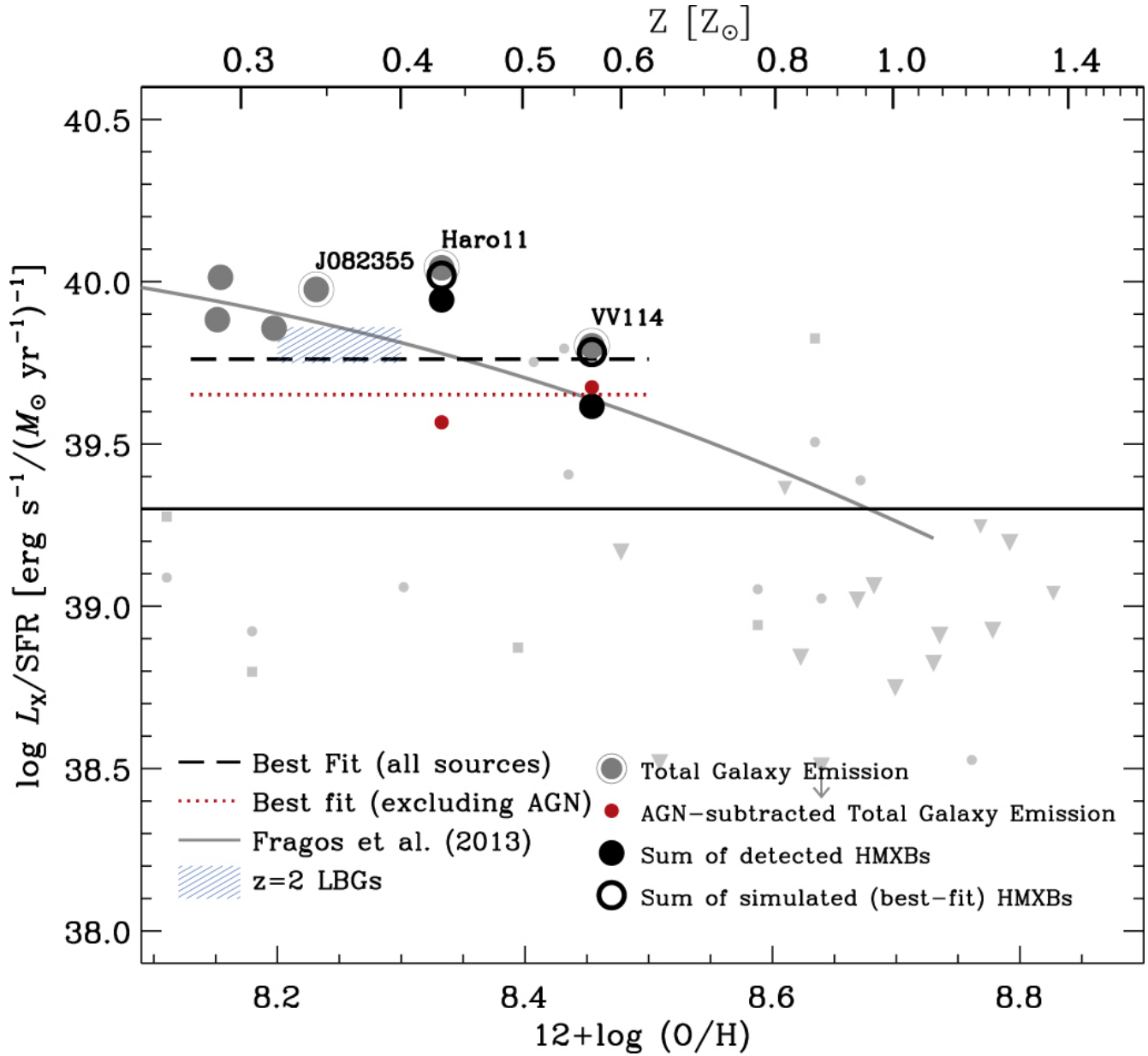
Figure 8. from EXPLORING THE OVERABUNDANCE OF ULXs IN METAL- AND DUST-POOR LOCAL LYMAN BREAK ANALOGS null 2016 APJ 818 140 doi:10.3847/0004-637X/818/2/140 https://dx.doi.org/10.3847/0004-637X/818/2/140 © 2016. The American Astronomical Society. All rights reserved.
