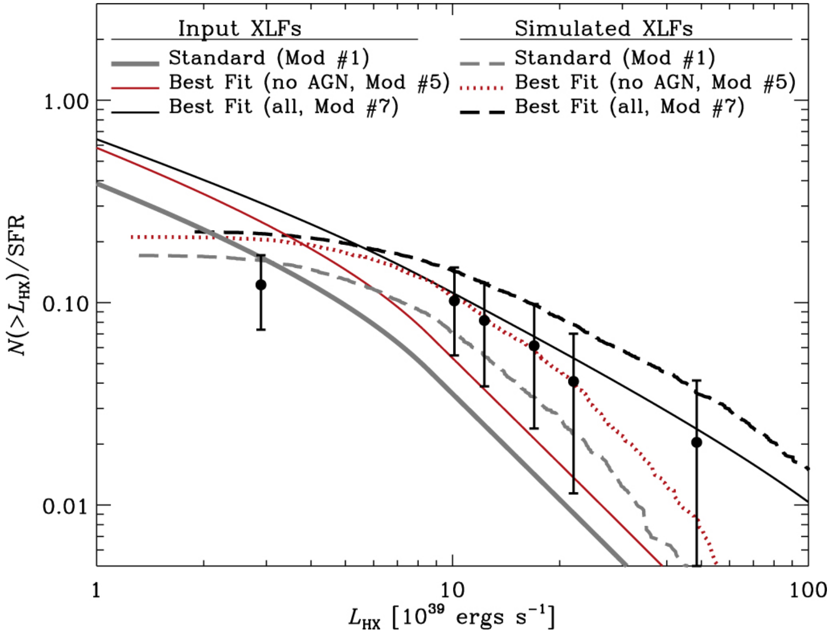
Figure 7. from EXPLORING THE OVERABUNDANCE OF ULXs IN METAL- AND DUST-POOR LOCAL LYMAN BREAK ANALOGS null 2016 APJ 818 140 doi:10.3847/0004-637X/818/2/140 https://dx.doi.org/10.3847/0004-637X/818/2/140 © 2016. The American Astronomical Society. All rights reserved.
