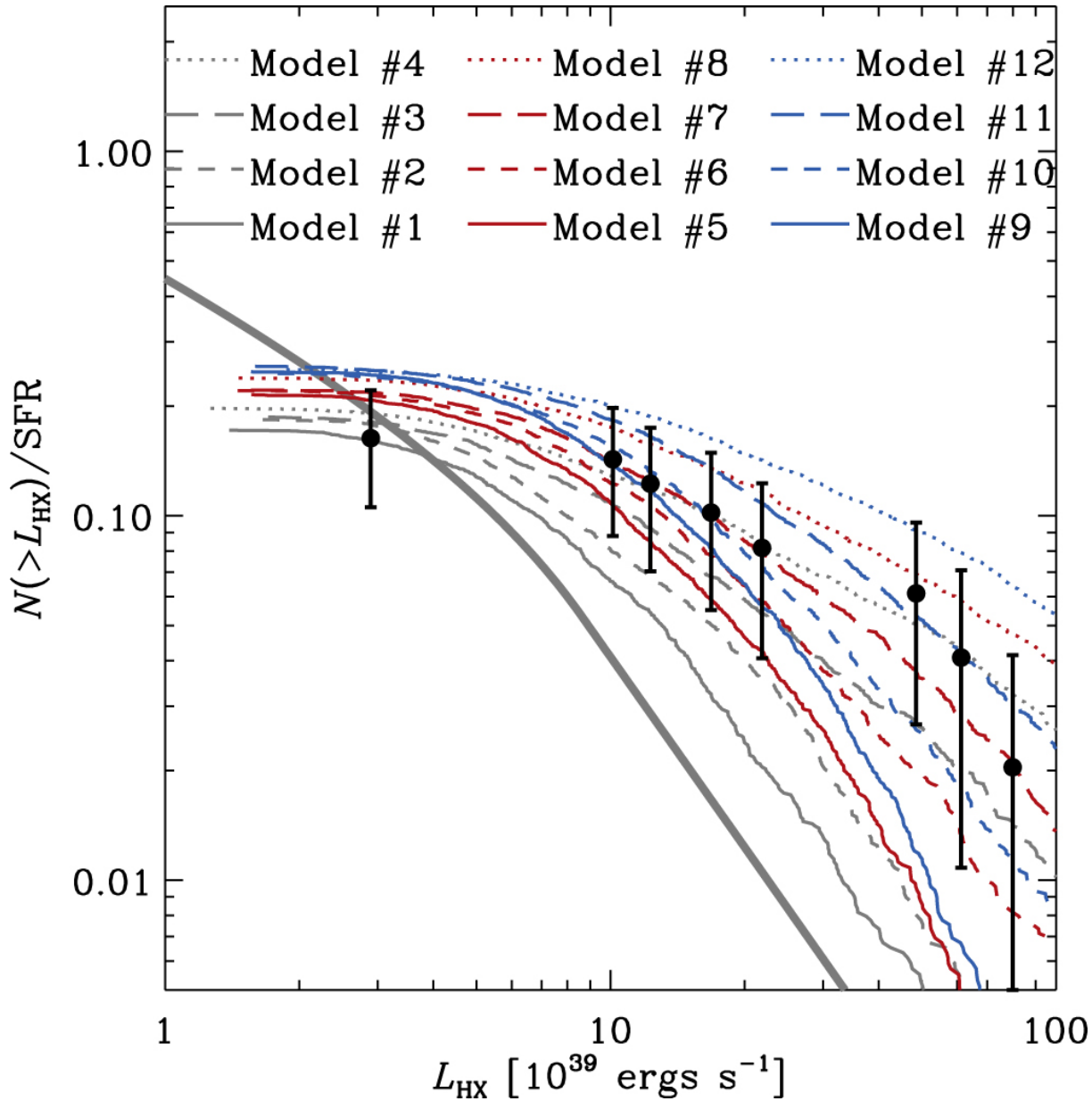
Figure 6. from EXPLORING THE OVERABUNDANCE OF ULXs IN METAL- AND DUST-POOR LOCAL LYMAN BREAK ANALOGS null 2016 APJ 818 140 doi:10.3847/0004-637X/818/2/140 https://dx.doi.org/10.3847/0004-637X/818/2/140 © 2016. The American Astronomical Society. All rights reserved.
