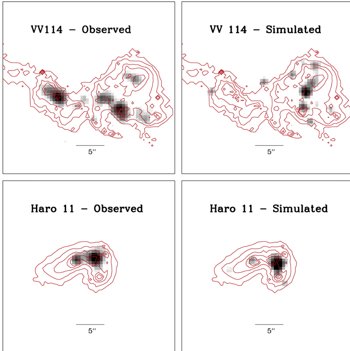
Figure 4. from EXPLORING THE OVERABUNDANCE OF ULXs IN METAL- AND DUST-POOR LOCAL LYMAN BREAK ANALOGS null 2016 APJ 818 140 doi:10.3847/0004-637X/818/2/140 https://dx.doi.org/10.3847/0004-637X/818/2/140 © 2016. The American Astronomical Society. All rights reserved.
