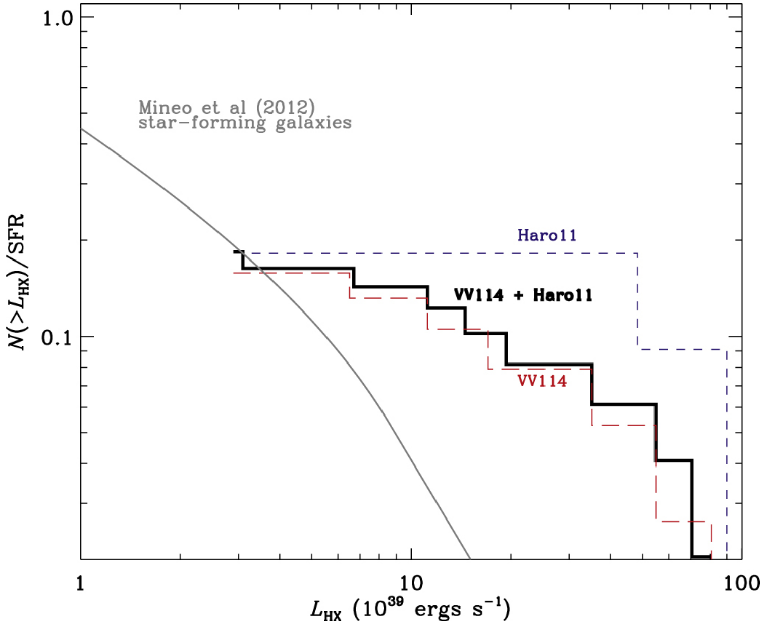
Figure 3. from EXPLORING THE OVERABUNDANCE OF ULXs IN METAL- AND DUST-POOR LOCAL LYMAN BREAK ANALOGS null 2016 APJ 818 140 doi:10.3847/0004-637X/818/2/140 https://dx.doi.org/10.3847/0004-637X/818/2/140 © 2016. The American Astronomical Society. All rights reserved.
