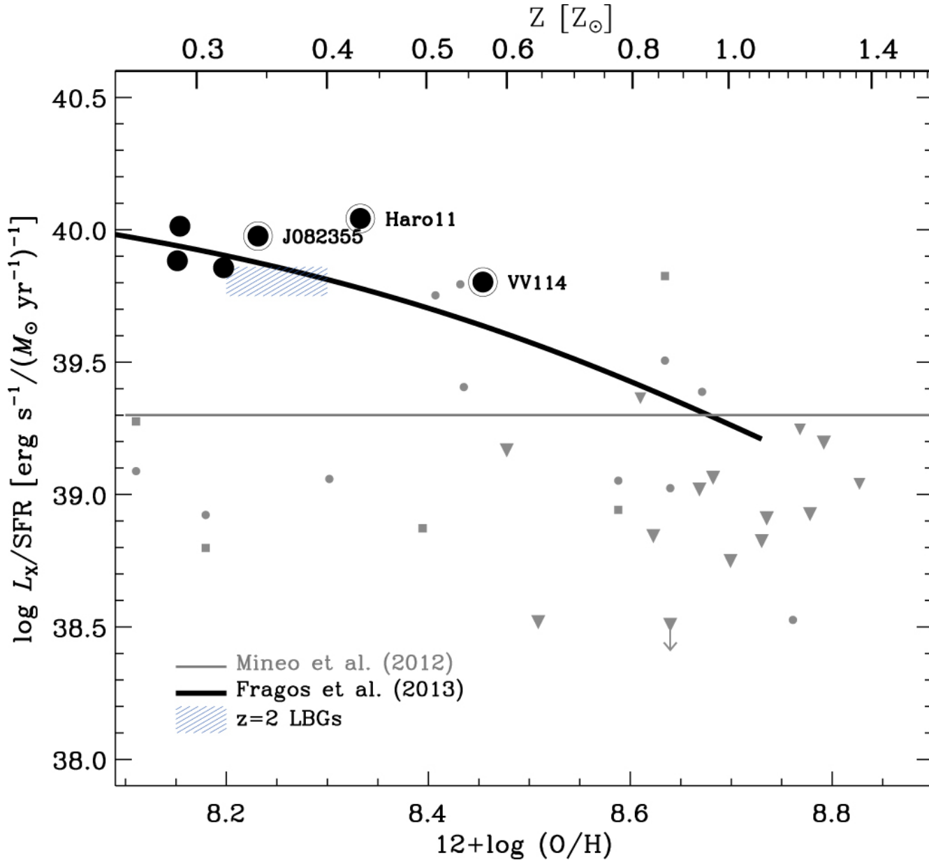
Figure 2. from EXPLORING THE OVERABUNDANCE OF ULXs IN METAL- AND DUST-POOR LOCAL LYMAN BREAK ANALOGS null 2016 APJ 818 140 doi:10.3847/0004-637X/818/2/140 https://dx.doi.org/10.3847/0004-637X/818/2/140 © 2016. The American Astronomical Society. All rights reserved.
