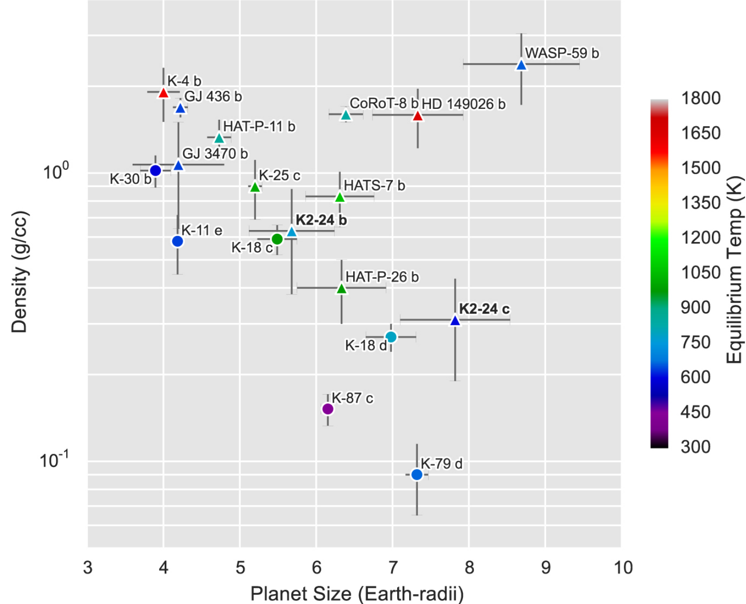
Figure 6. from TWO TRANSITING LOW DENSITY SUB-SATURNS FROM K2 null 2016 APJ 818 36 doi:10.3847/0004-637X/818/1/36 https://dx.doi.org/10.3847/0004-637X/818/1/36 © 2016. The American Astronomical Society. All rights reserved.
