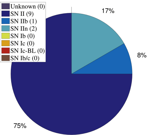
(c) Flash-Ionized Supernovae
