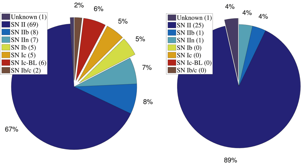
(a) All Core-Collapse Supernovae (b) Blue/Featureless Supernovae
