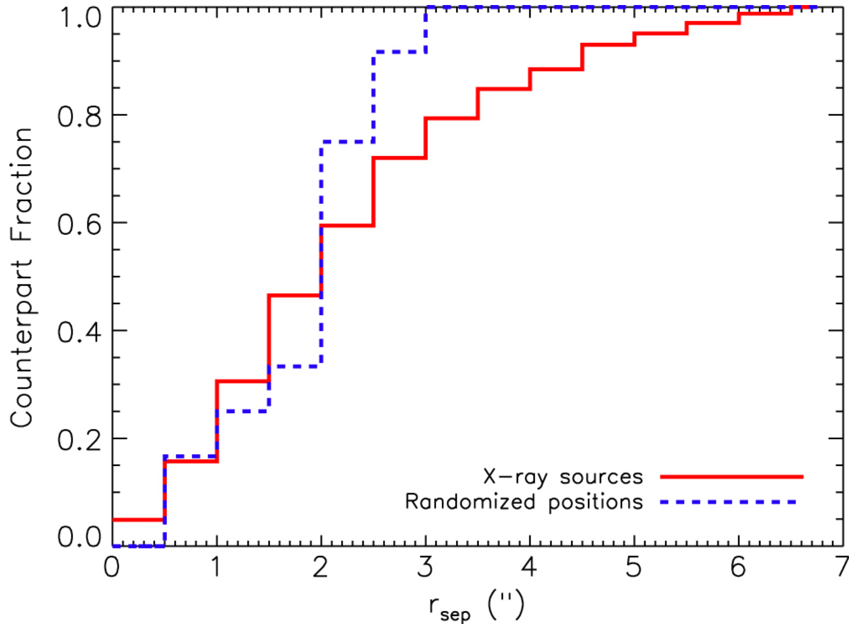
Figure 8. from THE 31 DEG2 RELEASE OF THE STRIPE 82 X-RAY SURVEY: THE POINT SOURCE CATALOG null 2016 APJ 817 172 doi:10.3847/0004-637X/817/2/172 https://dx.doi.org/10.3847/0004-637X/817/2/172 © 2016. The American Astronomical Society. All rights reserved.
